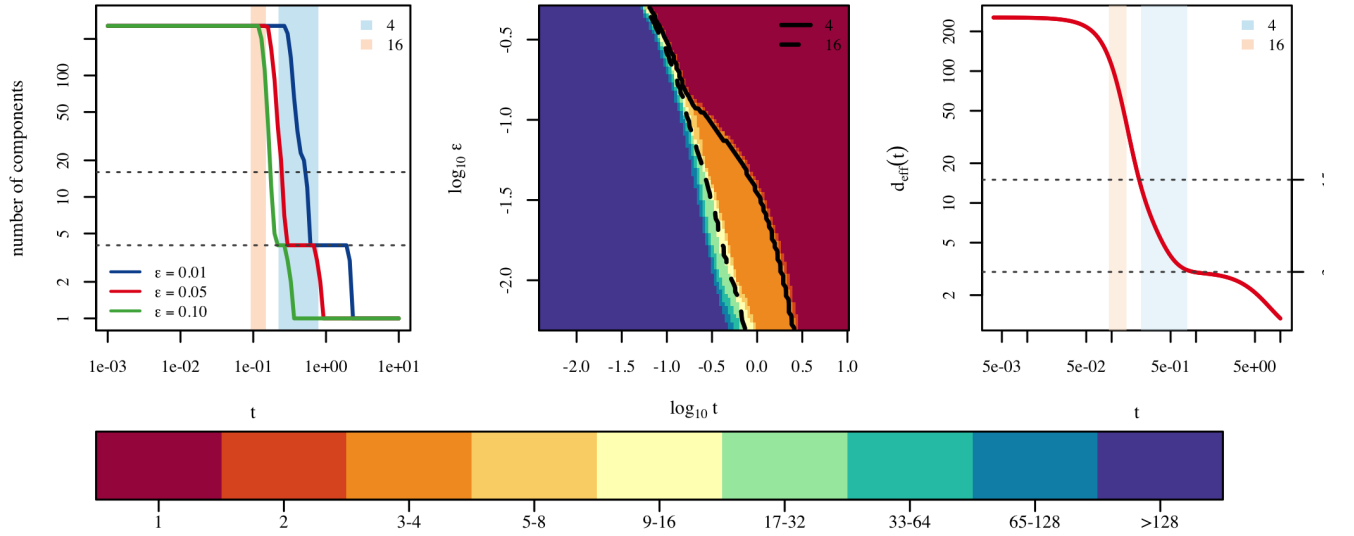
FIG. 4. Component count plateaus and diffusion geometry for the 13-4 network. Left: Component count n_{\text{comp}}(t) of the \varepsilon -thresholded diffusion network \mathcal{D}_T(t) for distance thresholds \varepsilon \in \{0.01, 0.05, 0.10\} using single-linkage clustering (SLINK), with shaded predicted spectral gap windows. Center: Contour map of n_{\text{comp}}(t, \varepsilon) over the logarithmic time-threshold plane ( t \in [0.004, 10] and \varepsilon \in [0.005, 0.50] ); nearly vertical contour lines confirm threshold-robustness of community detection, validating the SLINK method. Right: Effective embedding dimension d_{\text{eff}}(t) vs dynamic time t , displaying step-wise drops across the predicted 16-community and 4-community plateau windows.
