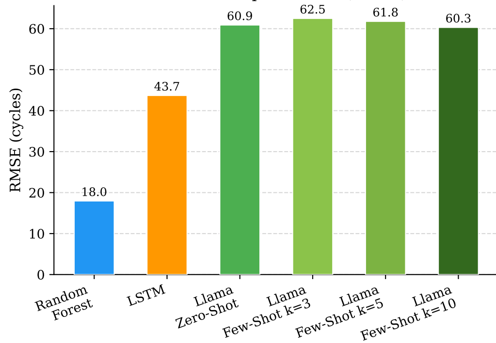
Root Mean Square Error (RMSE)
