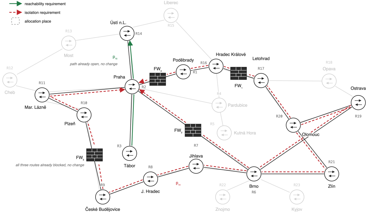
Figure 5.6: Iterations 4 and 5: p_{14} (Olomouc \nrightarrow Praha) is already blocked by FW_1 , FW_2 , and FW_3 on every route, and p_{15} (Tabor \rightarrow Usti n.L.) is already open, so neither requires a reconfiguration.
