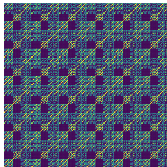
Correlation between test statistics
