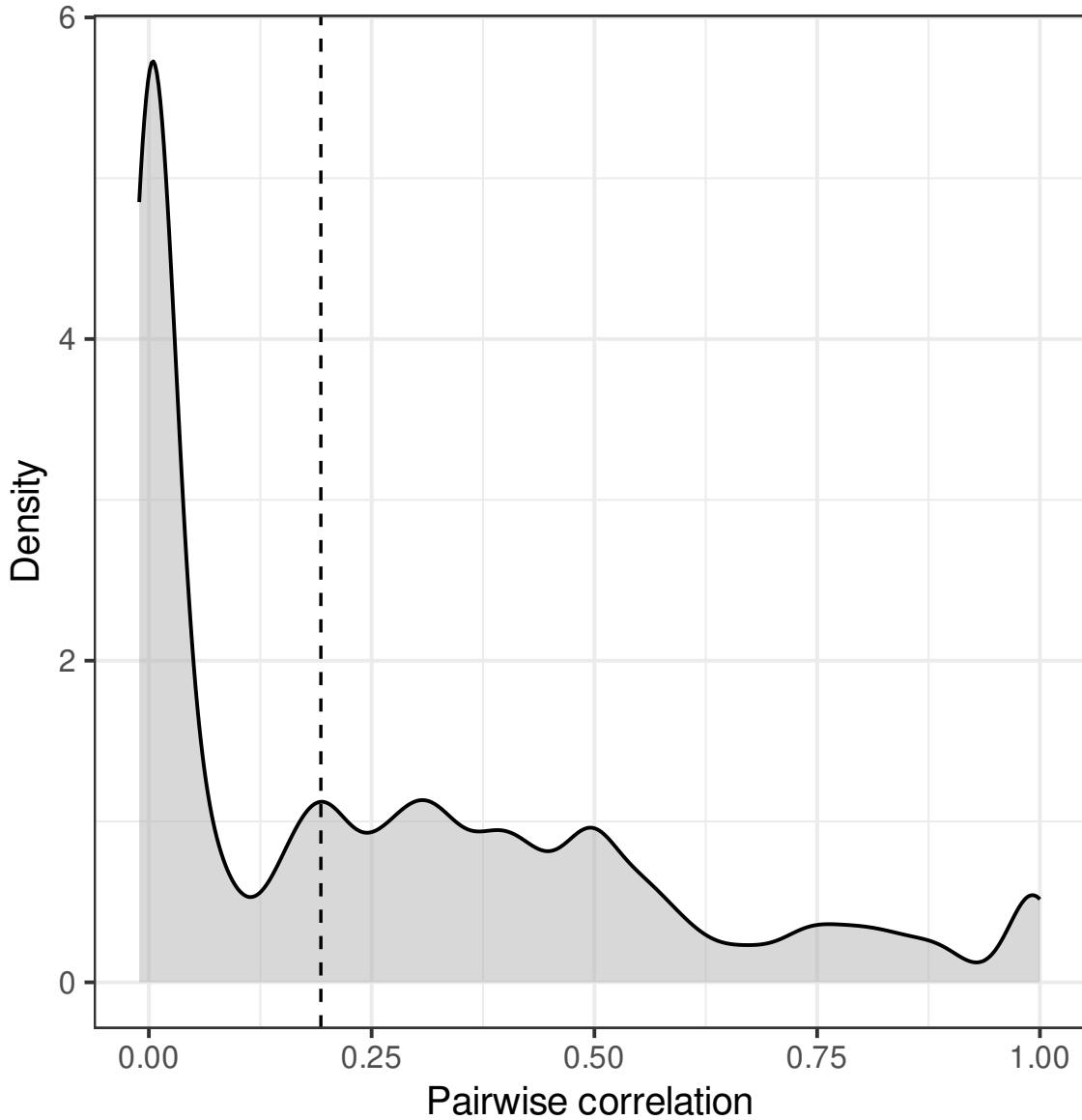
Distribution of pairwise correlations
