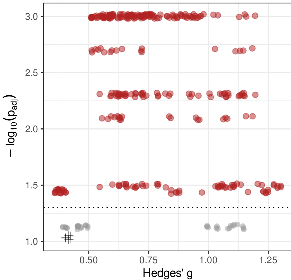
Volcano Plot
