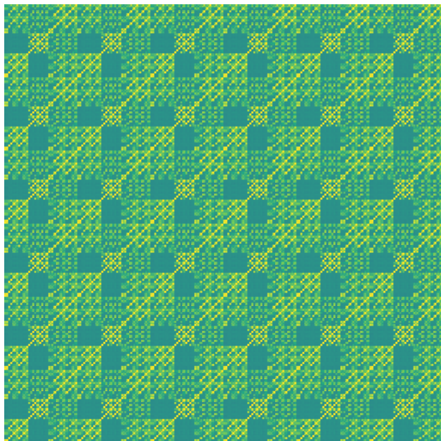
Pairwise correlation matrix
