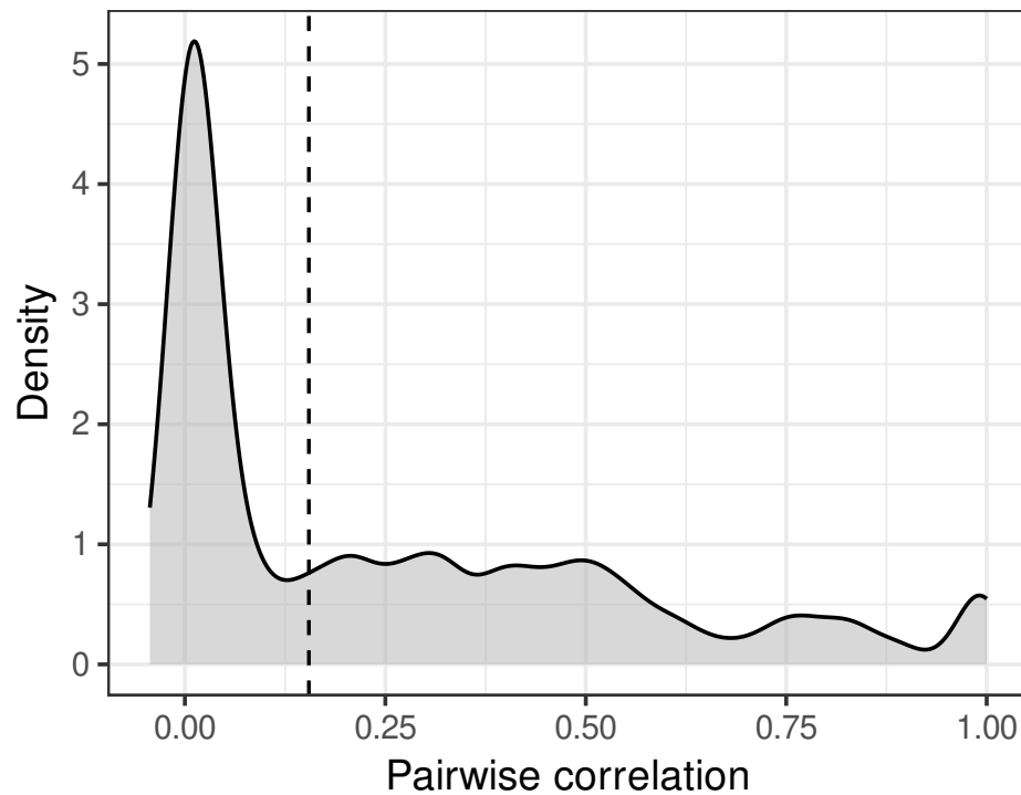
Distribution of pairwise correlations
