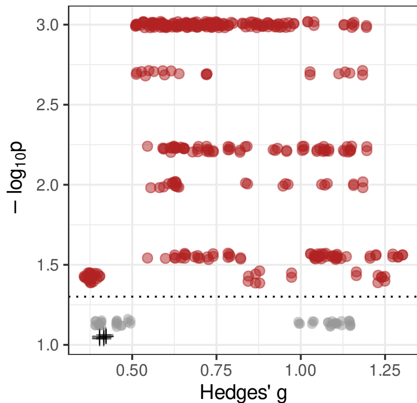
Volcano Plot
