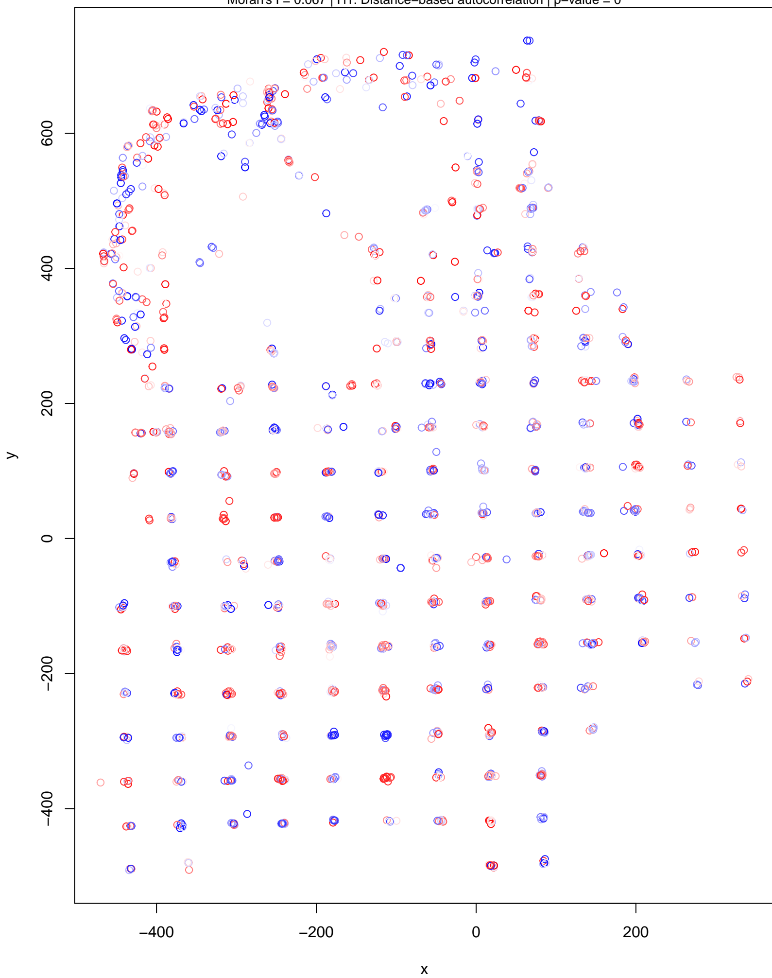
DHARMA Moran's I test for distance-based autocorrelation Moran's I = 0.067 | H1: Distance-based autocorrelation | p-value = 0
