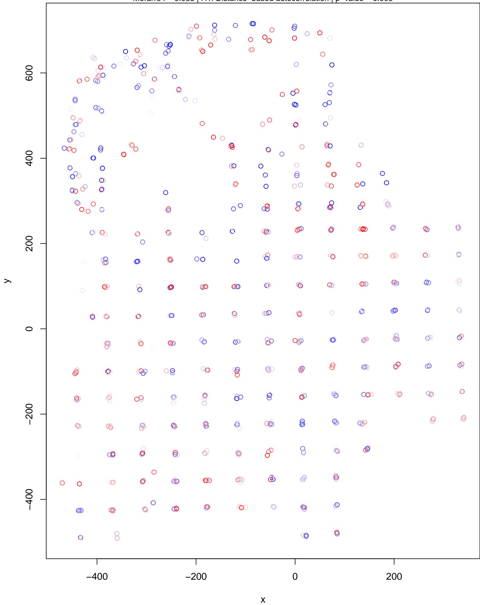
DHARMA Moran's I test for distance-based autocorrelation Moran's I = 0.038 | H1: Distance-based autocorrelation | p-value = 0.003
