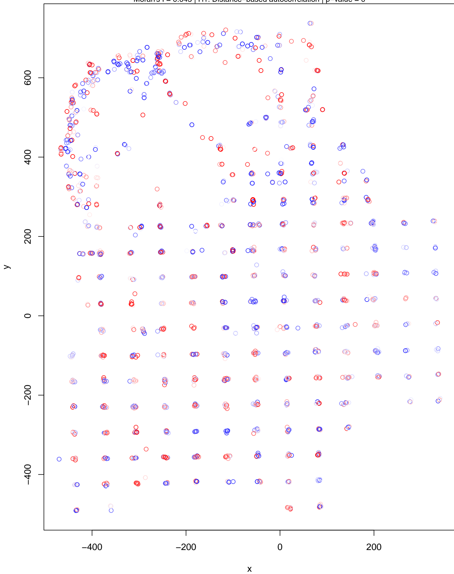
DHARma Moran's I test for distance-based autocorrelation Moran's I = 0.045 | H1: Distance-based autocorrelation | p-value = 0
