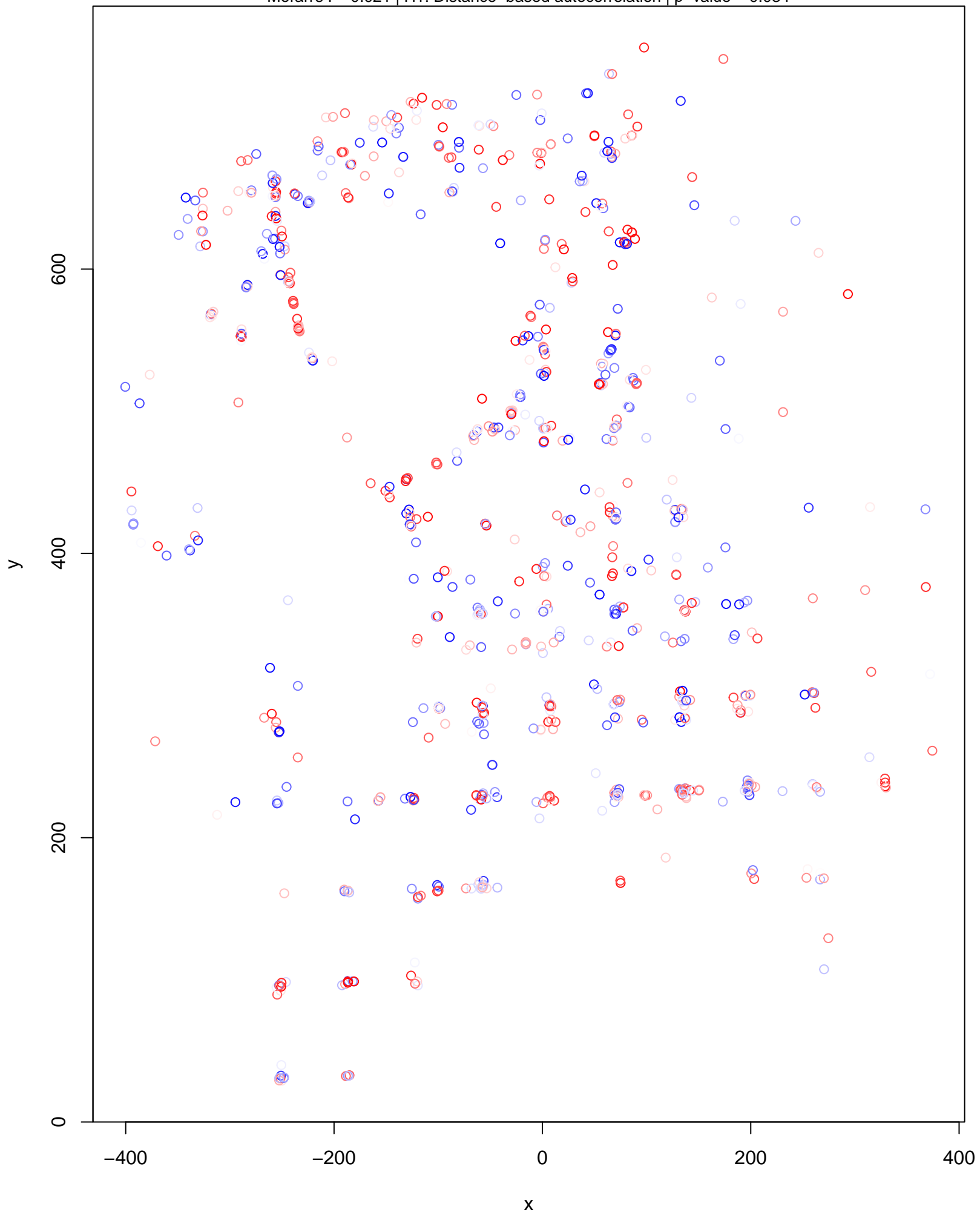
DHARMA Moran's I test for distance-based autocorrelation Moran's I = 0.021 | H1: Distance-based autocorrelation | p-value = 0.034
