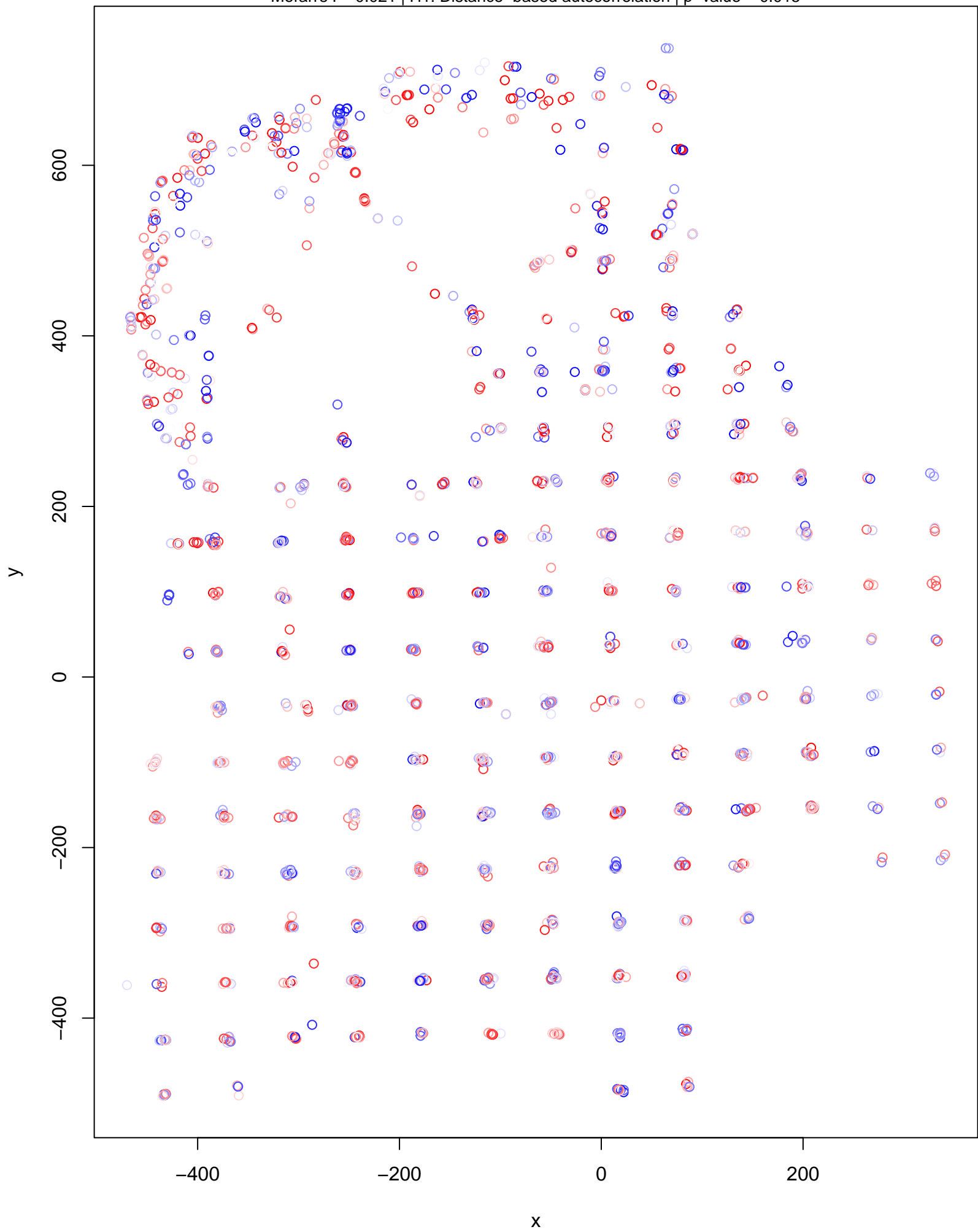
DHARma Moran's I test for distance-based autocorrelation Moran's I = 0.021 | H1: Distance-based autocorrelation | p-value = 0.015
