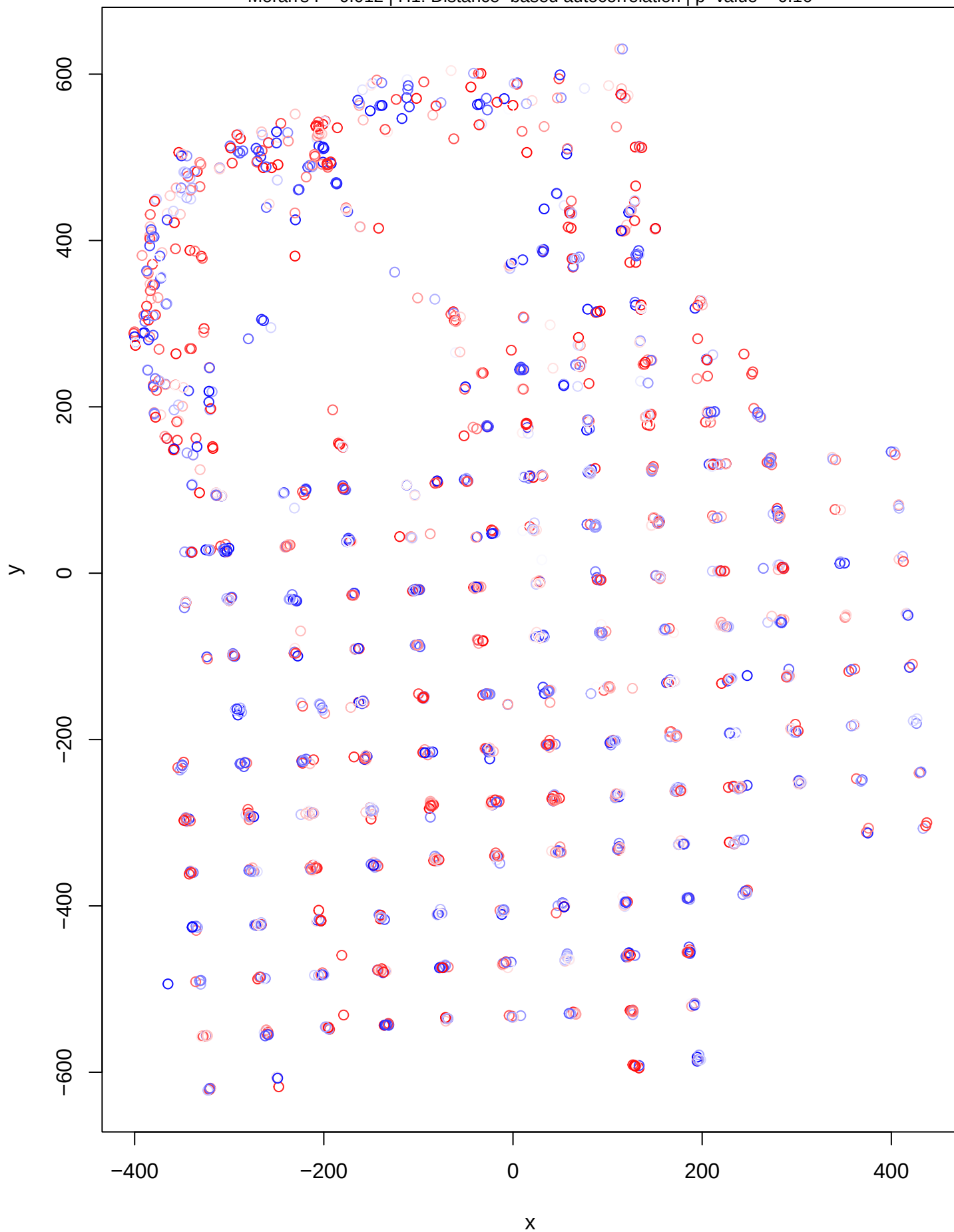
DHARMA Moran's I test for distance-based autocorrelation Moran's I = 0.012 | H1: Distance-based autocorrelation | p-value = 0.16
