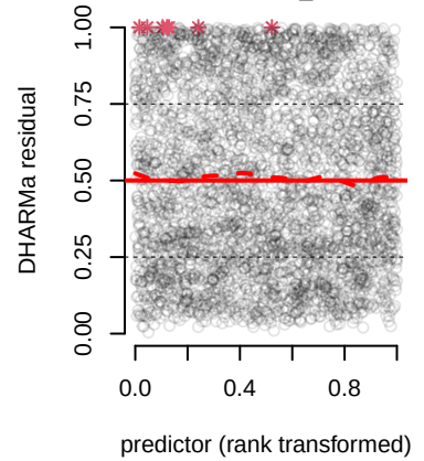
DHARMa residual Residual vs. pred
