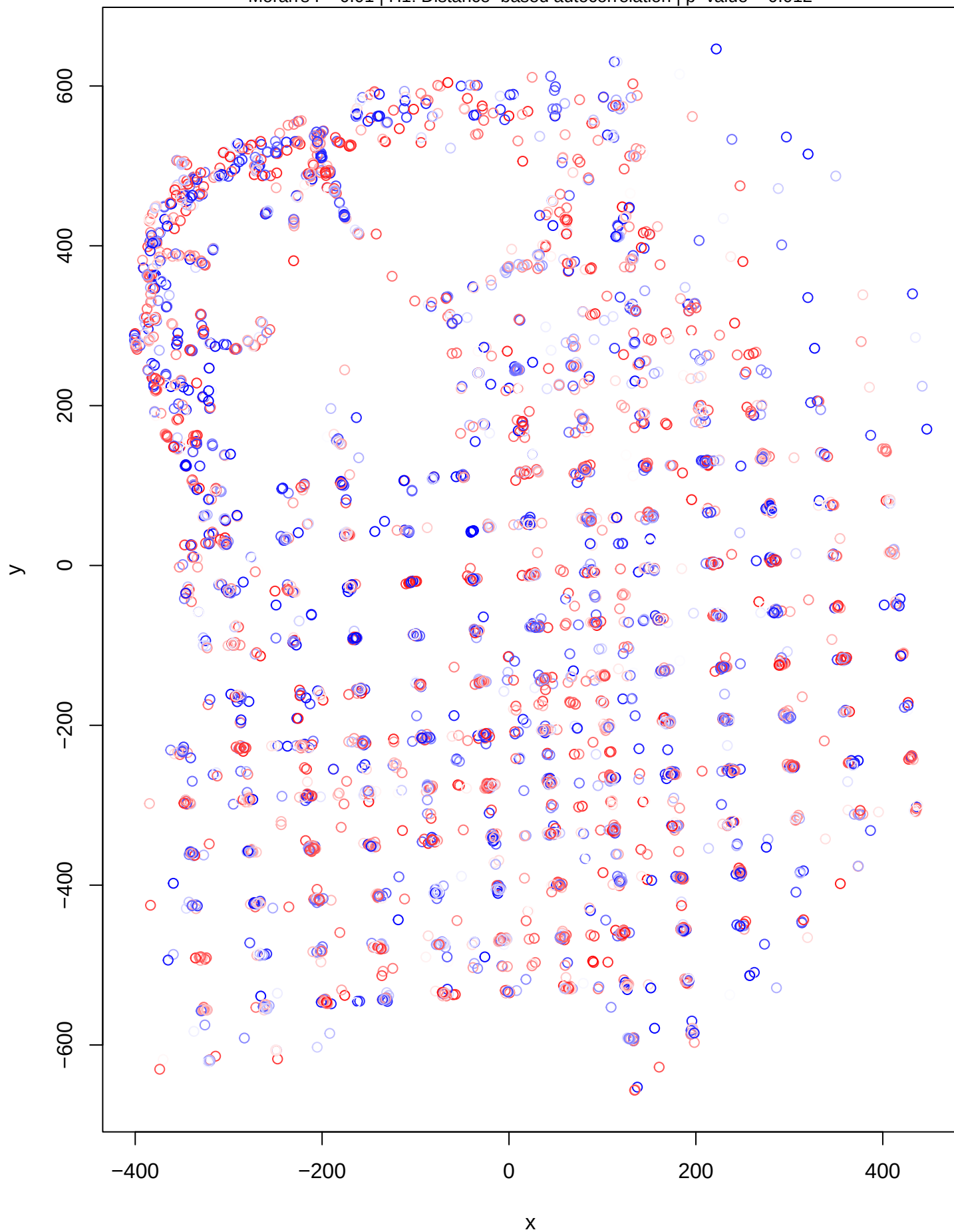
DHARMa Moran's I test for distance-based autocorrelation Moran's I = 0.01 | H1: Distance-based autocorrelation | p-value = 0.012
