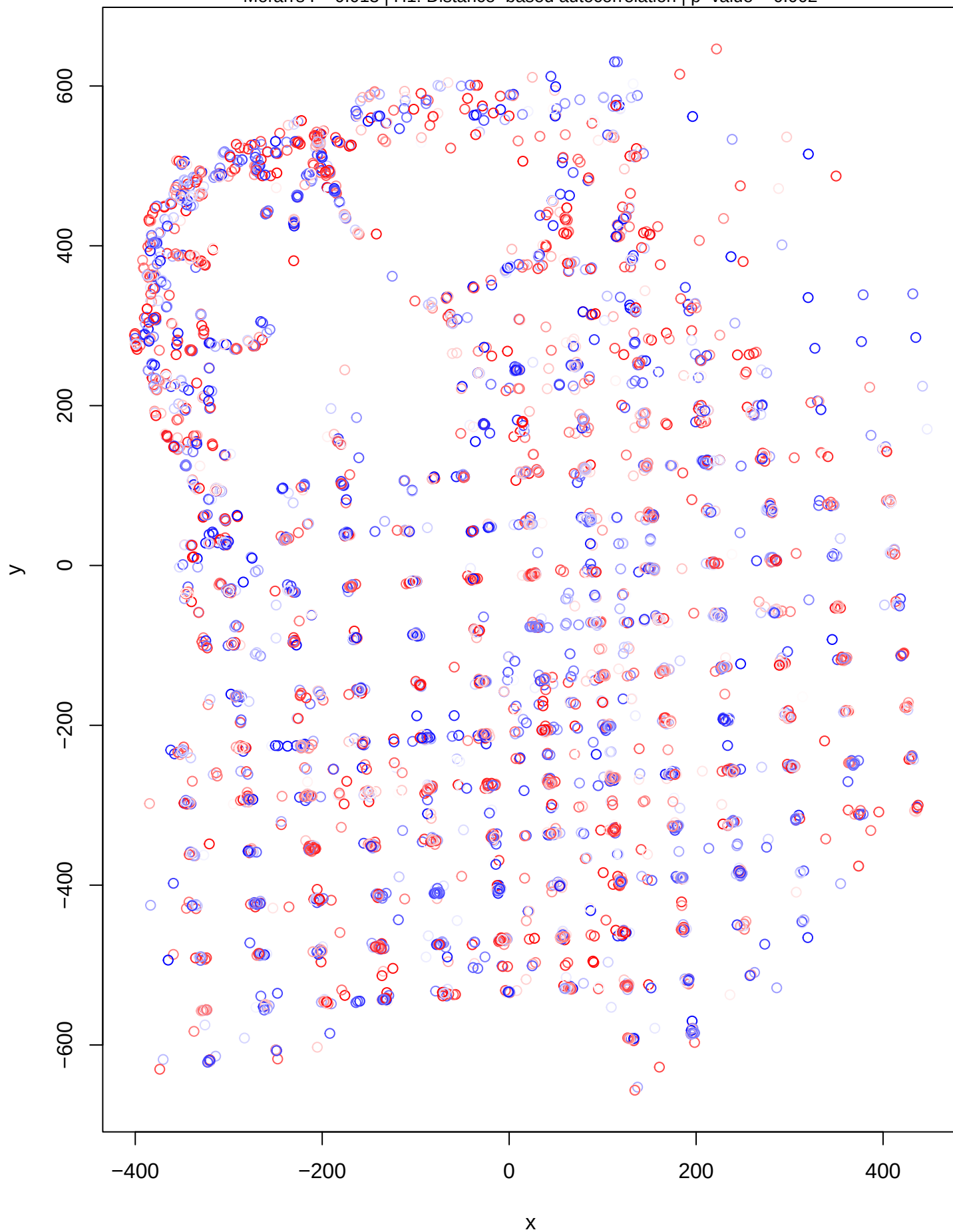
DHARMA Moran's I test for distance-based autocorrelation Moran's I = 0.013 | H1: Distance-based autocorrelation | p-value = 0.002
