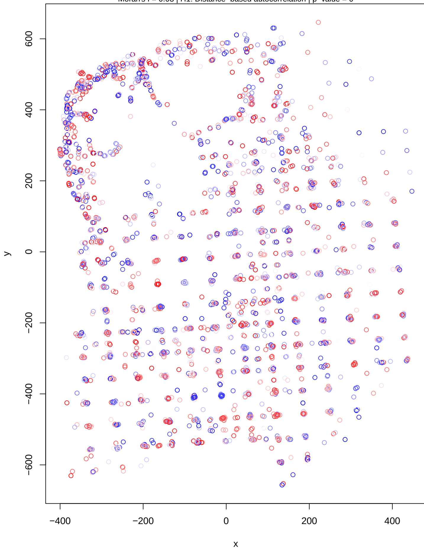
DHARMa Moran's I test for distance-based autocorrelation Moran's I = 0.03 | H1: Distance-based autocorrelation | p-value = 0
