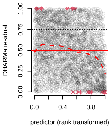
DHARMa residual Residual vs. pred
