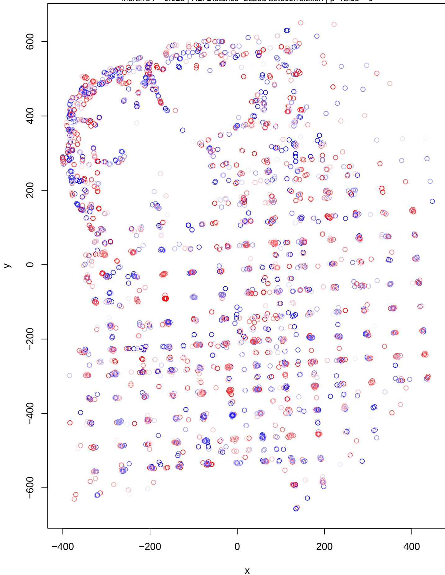
DHARMa Moran's I test for distance-based autocorrelation Moran's I = 0.028 | H1: Distance-based autocorrelation | p-value = 0
