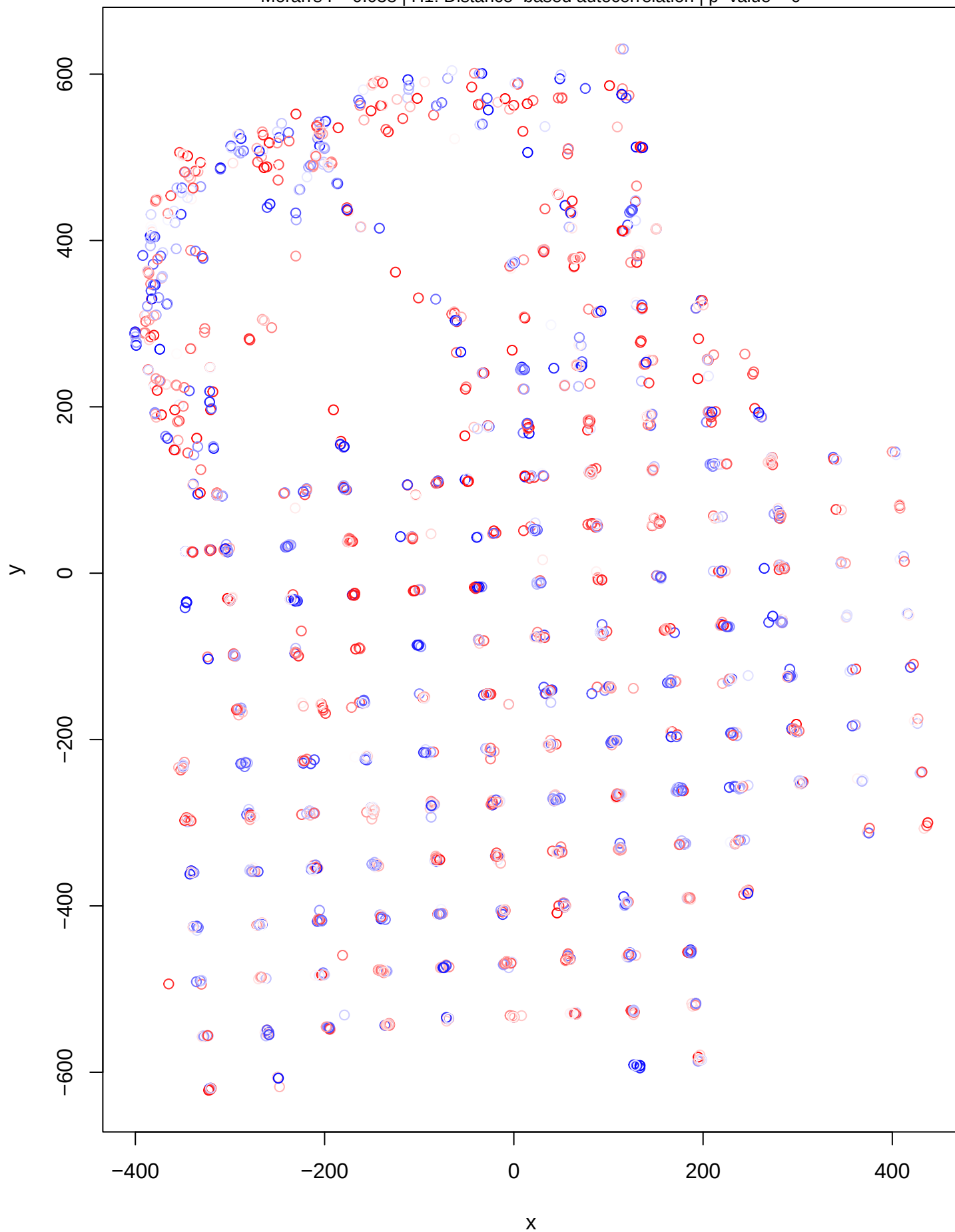
DHARMa Moran's I test for distance-based autocorrelation Moran's I = 0.038 | H1: Distance-based autocorrelation | p-value = 0
