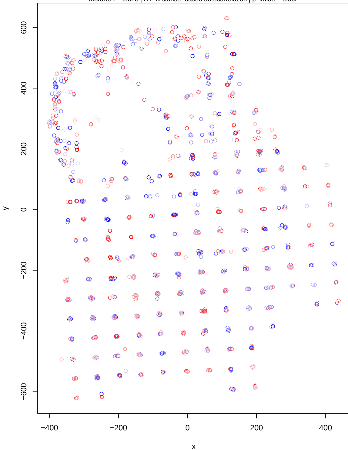
DHARMa Moran's I test for distance-based autocorrelation Moran's I = 0.028 | H1: Distance-based autocorrelation | p-value = 0.002
