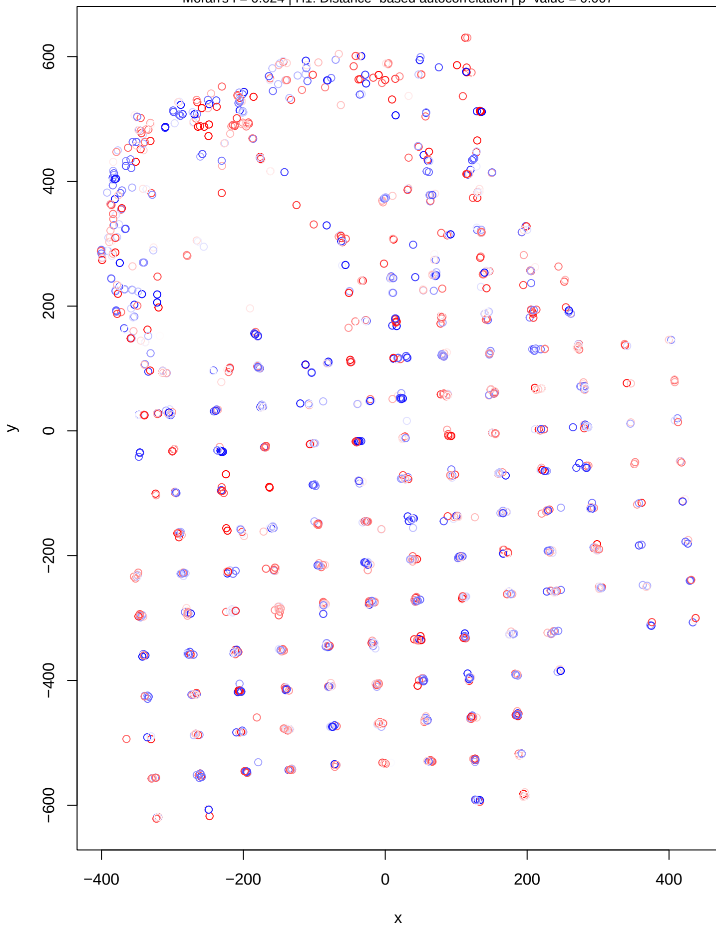
DHARMA Moran's I test for distance-based autocorrelation Moran's I = 0.024 | H1: Distance-based autocorrelation | p-value = 0.007
