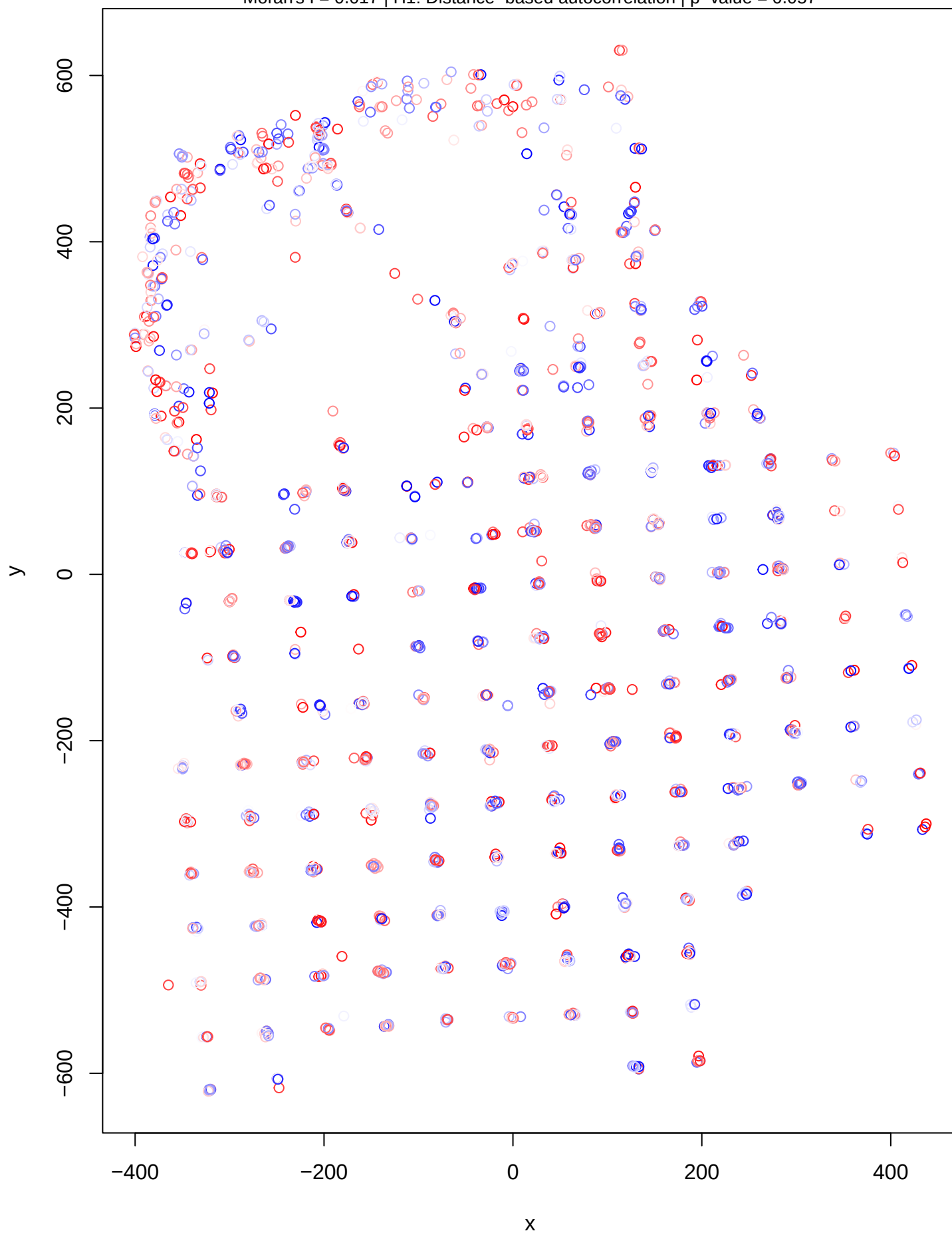
DHARMa Moran's I test for distance-based autocorrelation Moran's I = 0.017 | H1: Distance-based autocorrelation | p-value = 0.057
