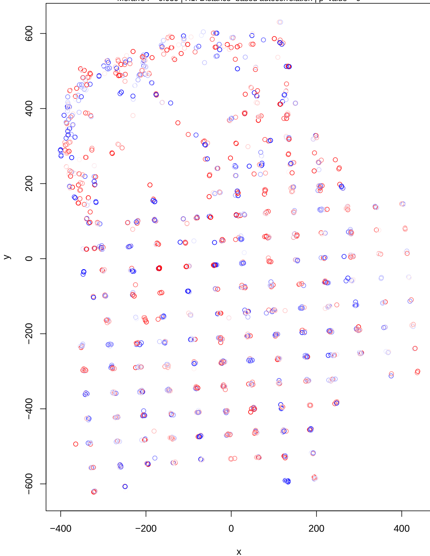
DHARMA Moran's I test for distance-based autocorrelation Moran's I = 0.039 | H1: Distance-based autocorrelation | p-value = 0
