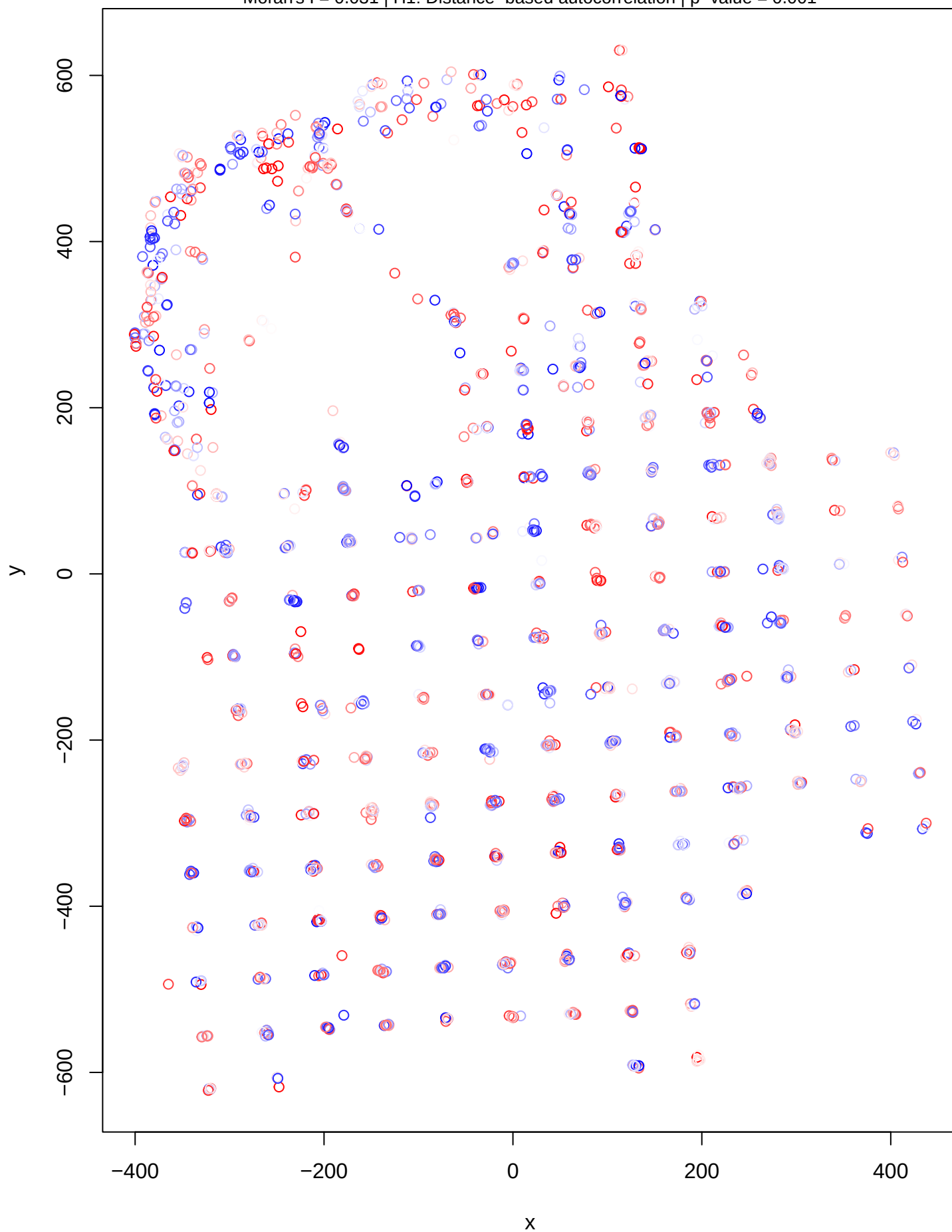
DHARMA Moran's I test for distance-based autocorrelation Moran's I = 0.031 | H1: Distance-based autocorrelation | p-value = 0.001
