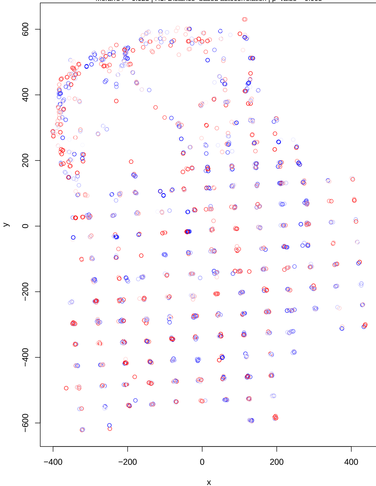
DHARMA Moran's I test for distance-based autocorrelation Moran's I = 0.025 | H1: Distance-based autocorrelation | p-value = 0.005
