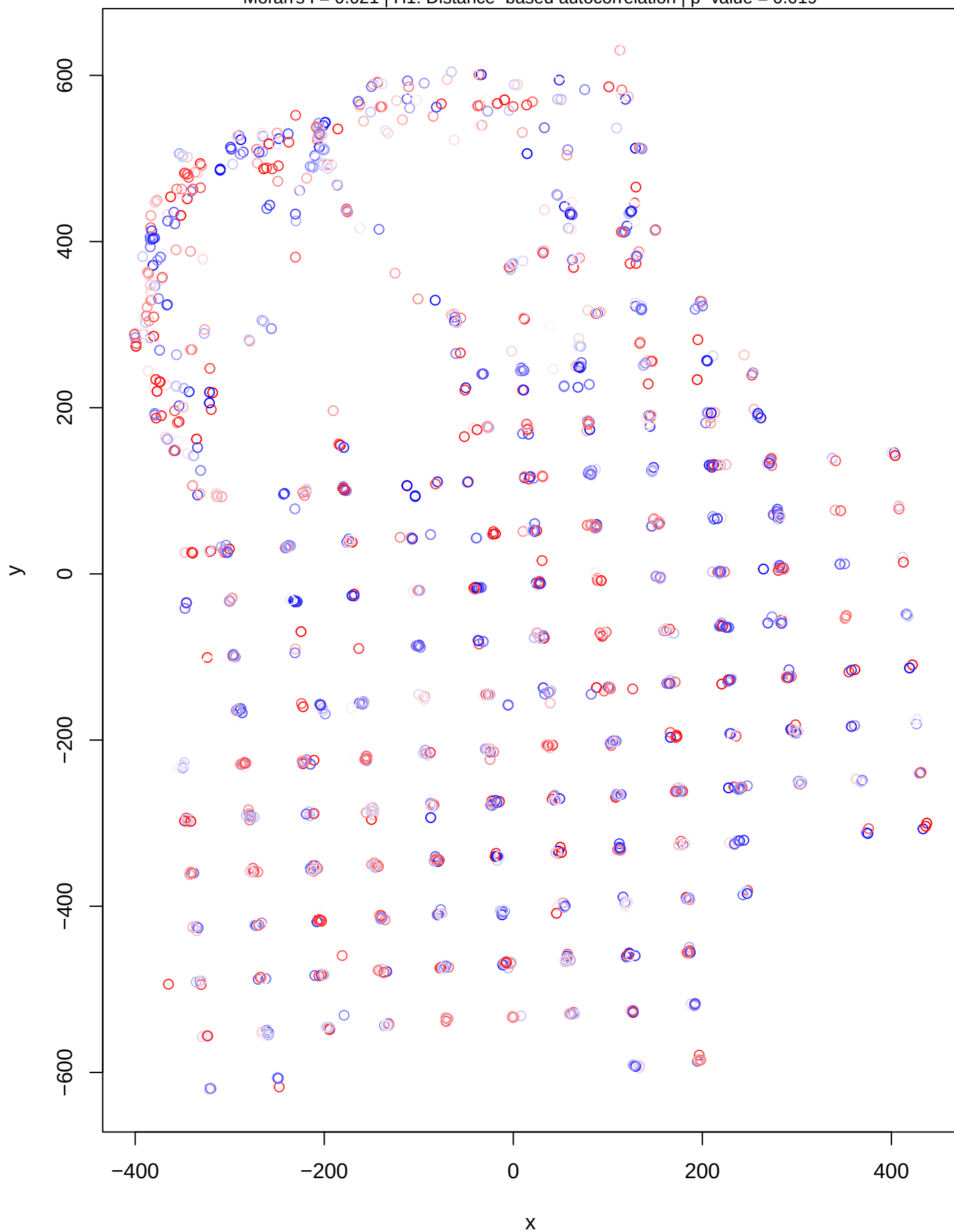
DHARMa Moran's I test for distance-based autocorrelation Moran's I = 0.021 | H1: Distance-based autocorrelation | p-value = 0.019
