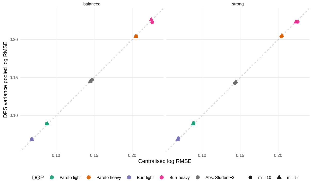
Figure 4.1: Log RMSE of the pooled estimator using the variance weights of Daouia et al. (2024) against the centralised benchmark in the main grid with k_j/n_j = 0.05 and np = 5 . The dashed line is equality. Points near the line indicate that the pooled route tracks the centralised benchmark closely.
