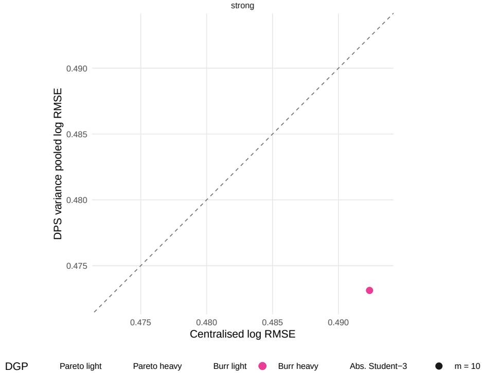
Figure 4.1: Log RMSE of the DPS variance pooled estimator against the centralised benchmark in the main grid with k_j/n_j = 0.05 and np = 5 . The dashed line is equality. Points near the line indicate that the pooled route tracks the centralised benchmark closely.
