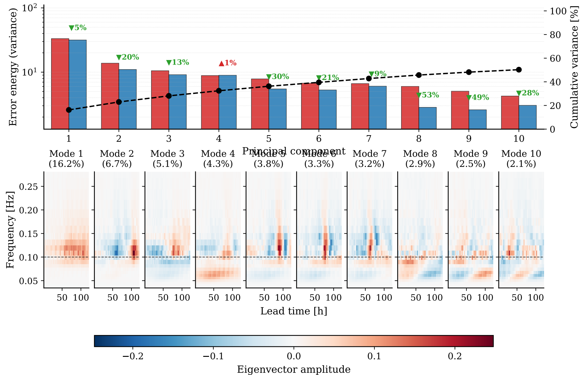
(a) PCA scree and cumulative variance
