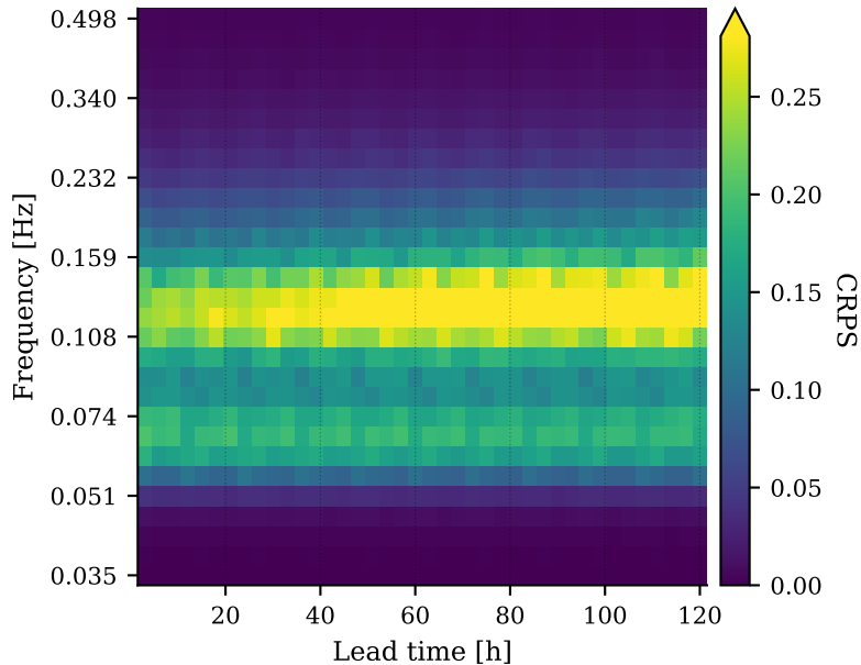
(a) Probabilistic error (CRPS)
