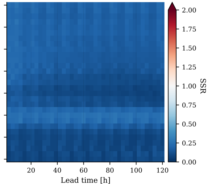
(b) Ensemble spread / RMSE (SSR)
