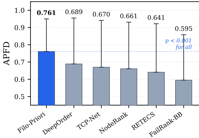
(a) Industrial QTA (277 builds)
