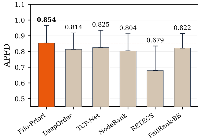
(b) RTPTorrent (20 projects)
