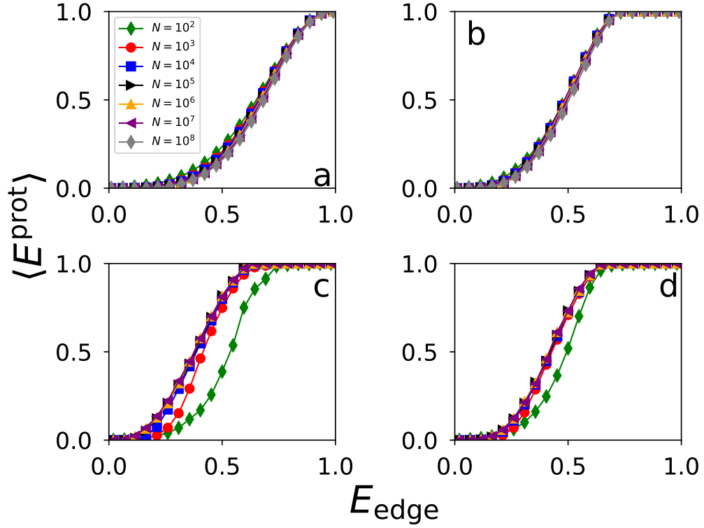
Figure S6. Quantum communication on synthetic networks. (a) We plot the average entanglement \langle E^{\text{CPA}} \rangle as a function of the entanglement of the individual edges E_{\text{edge}} for network generated according to the configuration model with degree exponent \gamma = 2.1 . Different symbols and colors correspond to different network sizes. (b-d) Same as in (a), but for QPA, h1QPA and h2QPA, respectively.
