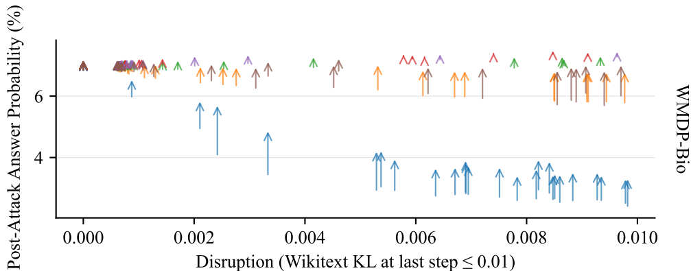
Qwen3.5-9B
