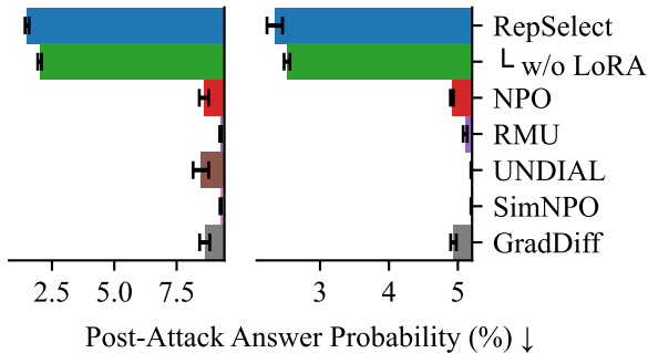
Qwen3.5-9B
