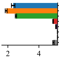
Qwen3.5-9B
