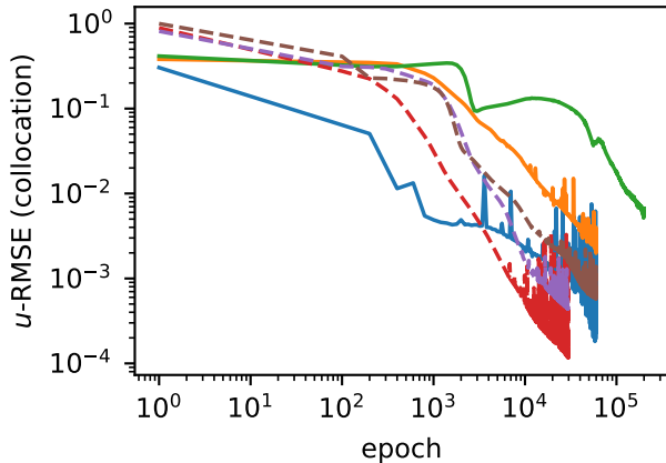
(b) solution error vs exact soliton
