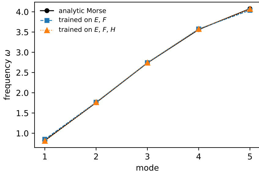
phonons of the equilibrium chain
