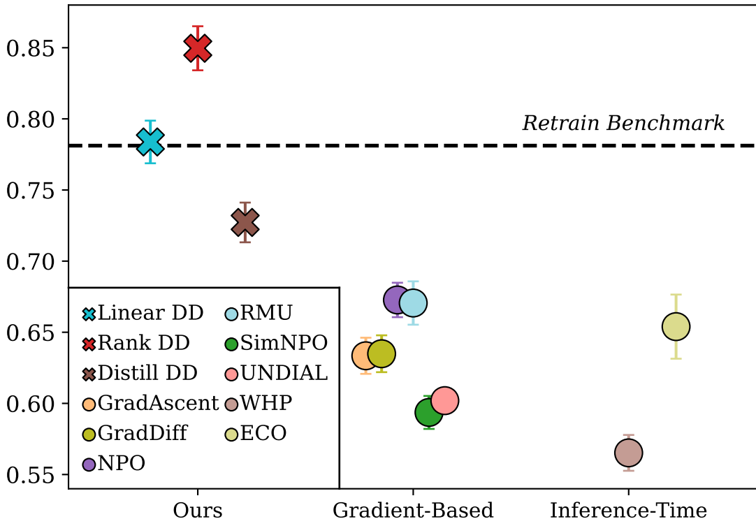
TOFU Aggregate Score
