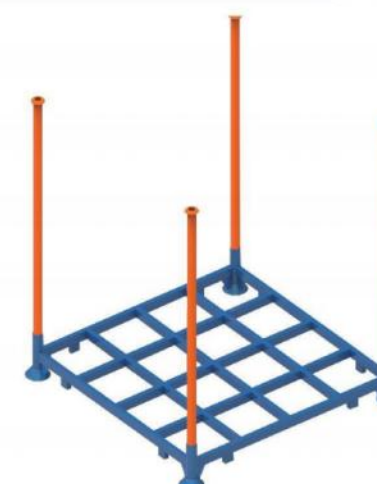
BSD-F-B furniture stacking rack
