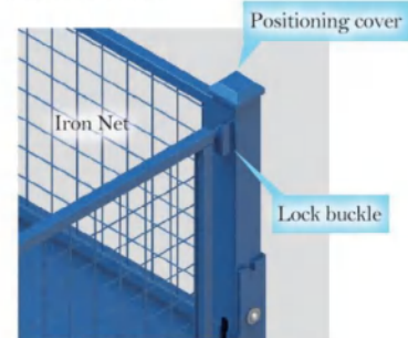
■ Structural schematic
