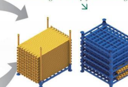
Schematic diagram of empty rack stacking
