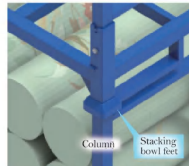
Connection diagram
