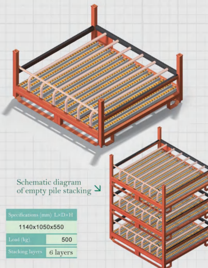
BSD-D-B Battery stacking cage
