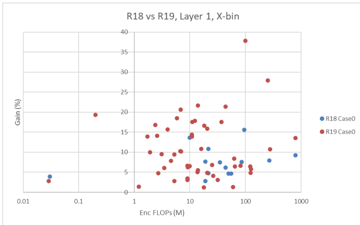
Figure 6.2.2.18-9: SGCS gain vs. encoder FLOPs, comparing the numbers from CSI_Table 1 (Rel-18) and the numbers from CSI_Table X9 (Rel-19)
