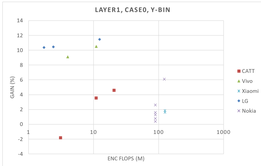
Figure 6.2.2.18-2: Case 0, encoder complexity (FLOPs) vs. SGCS gain (Y-bin)
