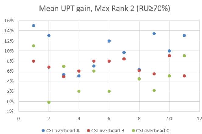
Figure 6.2.2.8-8: Mean UPT gain, Max Rank 2 ( RU \geq 70\% ), x-axis means index of source
