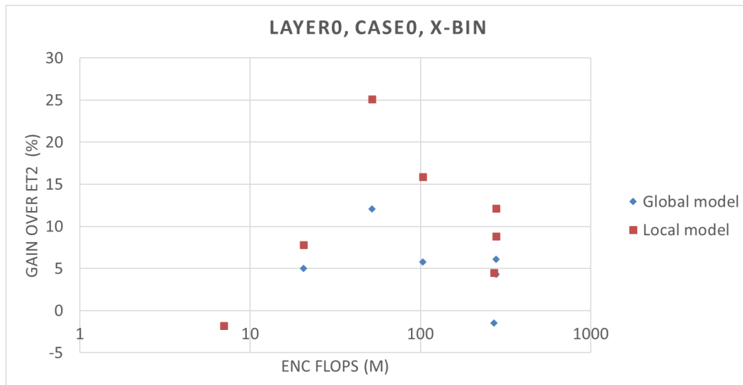
Figure 6.2.2.18-17: Case 0 model complexity (FLOPs) vs. SGCS gain for global and local models
