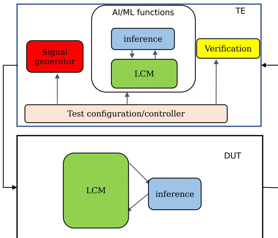
Figure 7.3.2.3-2: Reference block diagram for 2-sided model
