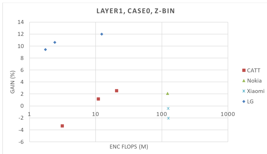
Figure 6.2.2.18-3: Case 0, encoder complexity (FLOPs) vs. SGCS gain (Z-bin)
