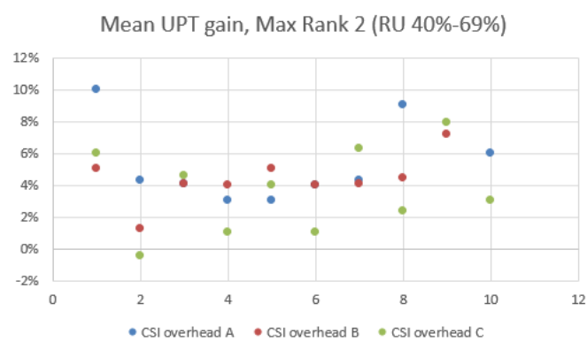
Figure 6.2.2.8-5: Mean UPT gain, Max Rank 2 (RU40%-69%), x-axis means index of source
