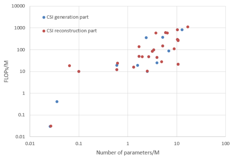
Figure 6.2.2.1-1: Complexity of AI/ML models from evaluation results in terms of FLOPs and number of parameters for CSI compression
