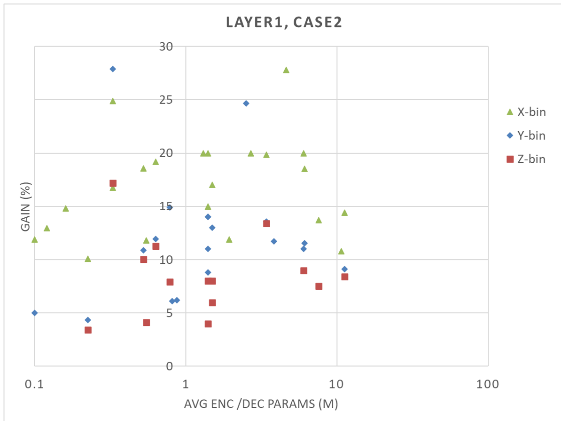
Figure 6.2.2.18-11: Case 2, model size (#parameters) vs. SGCS gain
