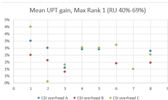
Figure 6.2.2.8-4: Mean UPT gain, Max Rank 1 (RU40%-69%), x-axis means index of source
