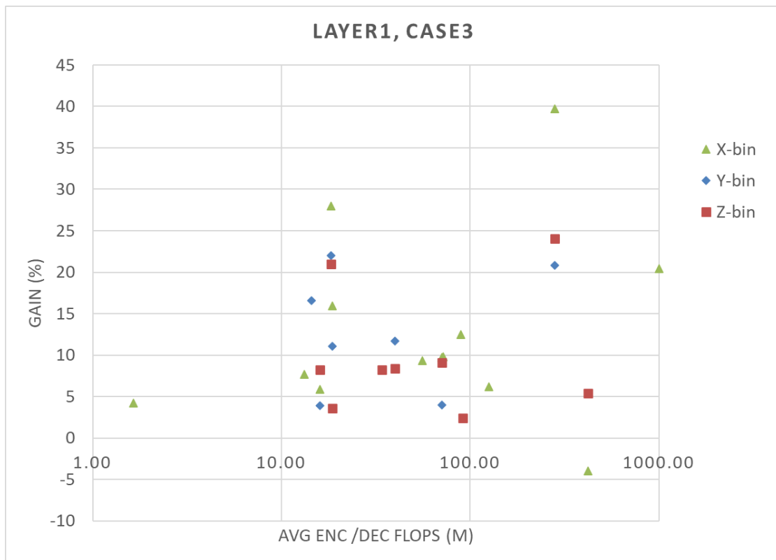
Figure 6.2.2.18-14: Case 3, model complexity (FLOPs) vs. SGCS gain
