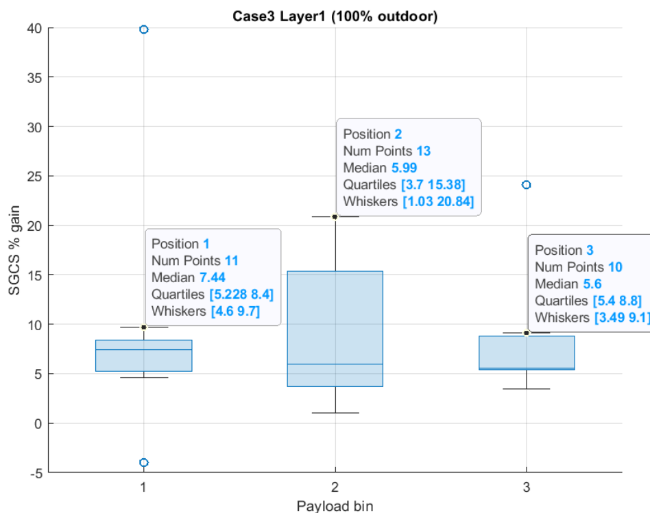
Figure 6.2.2.10-2: SGCS gain Case 3, Layer 1 for 100% outdoor
