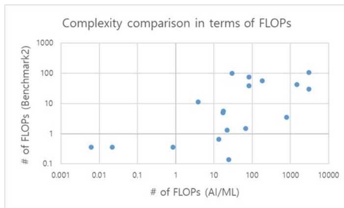
Figure 6.2.2.6A-2: Complexity of AI/ML models and benchmark 2 of an auto-regression/Kalman filter from evaluation results in terms of FLOPs for CSI prediction.
