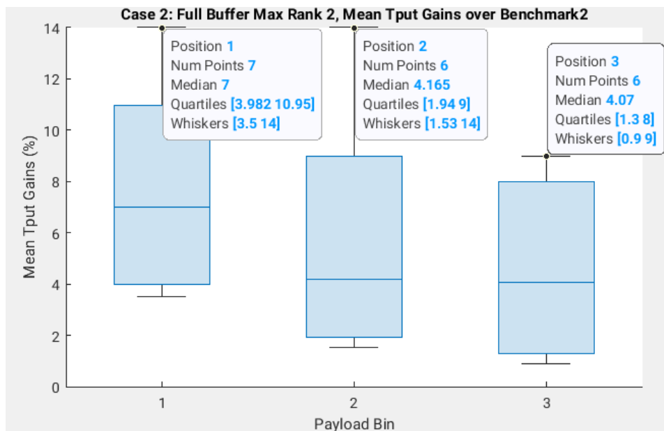
Figure 6.2.2.9-10: Mean Throughput gains over Benchmark 2, for Bins A, B and C, for Max Rank =2.
