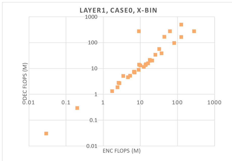
Figure 6.2.2.18-7: Decoder complexity vs. Encoder complexity (#FLOPS)
