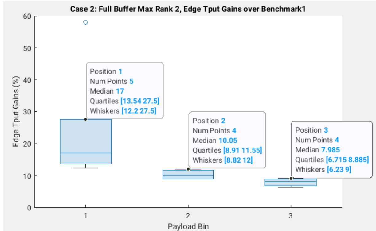
Figure 6.2.2.9-11: Edge Throughput gains over Benchmark 1, for Bins A, B and C, for Max Rank =2
