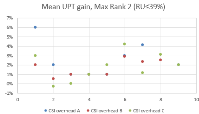
Figure 6.2.2.8-2: Mean UPT gain, Max Rank 2 (RU≤39%), x-axis means index of source
