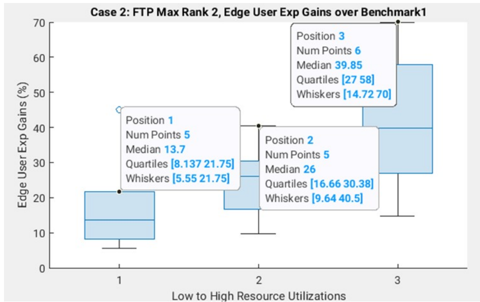
Figure 6.2.2.9-7: Edge User Exp Gains over benchmark 1 (FTP Max Rank 2)
