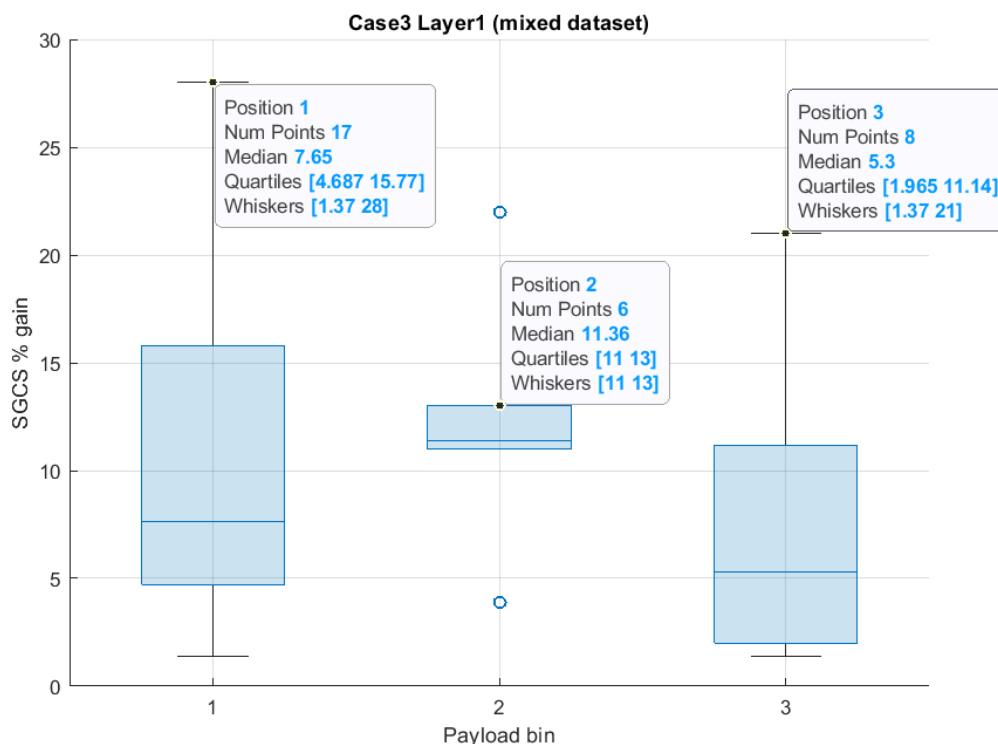
Figure 6.2.2.10-1: SGCS gain Case 3, Layer 1 for mixed dataset
