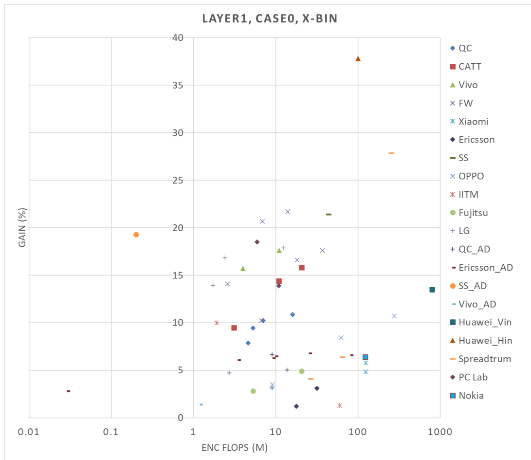
Figure 6.2.2.18-1: Case 0, encoder complexity (FLOPs) vs. SGCS gain (X-bin)
