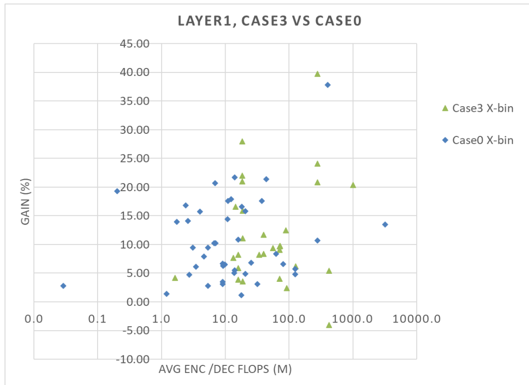
Figure 6.2.2.18-16: Case 0 compared to Case 3 in terms of complexity vs. performance
