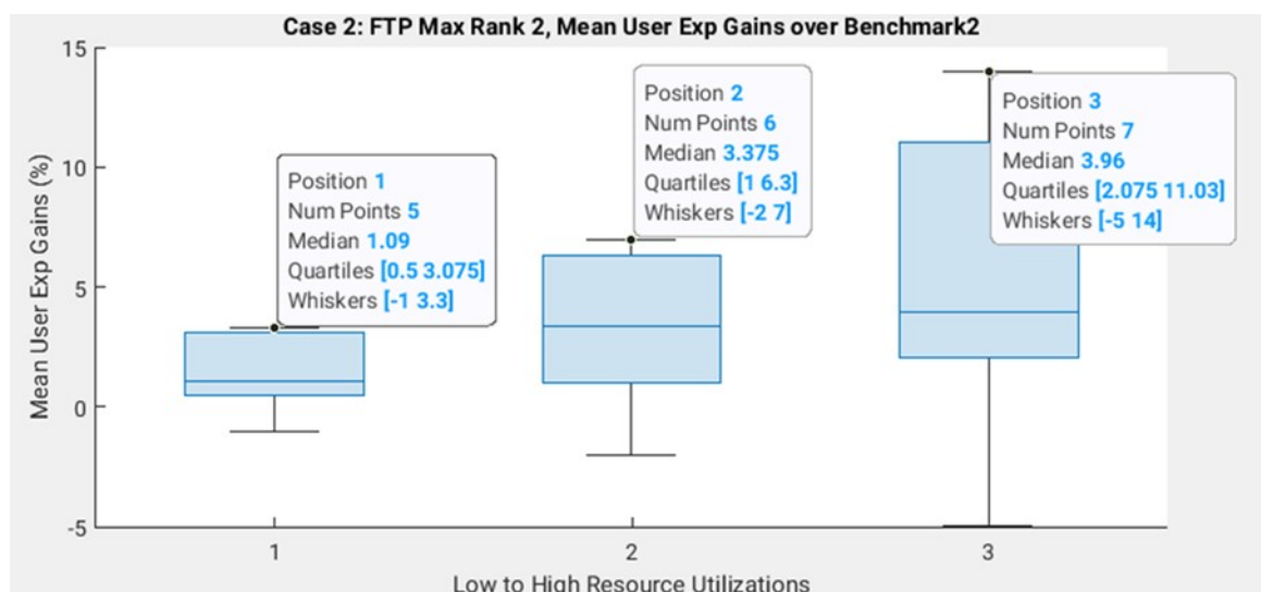
Figure 6.2.2.9-6: Mean User Exp Gains over benchmark 2 (FTP Max Rank 2)
