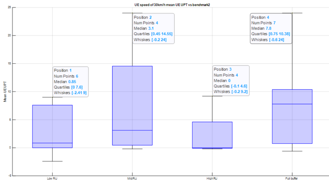
Figure 6.2.2.6A-3: Mean UPT distributions for full buffer with UE speed of 30km/h.
