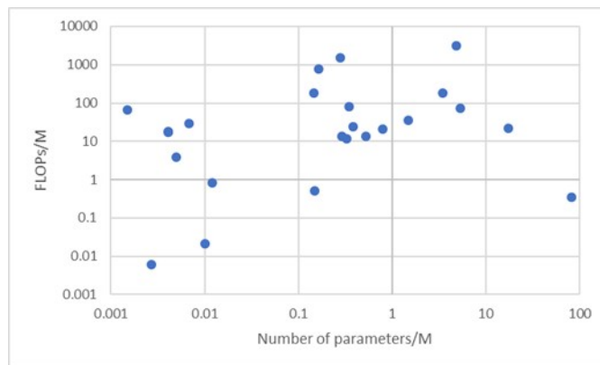
Figure 6.2.2.6A-1: Complexity of AI/ML models from evaluation results in terms of FLOPs and number of parameters for CSI prediction.
