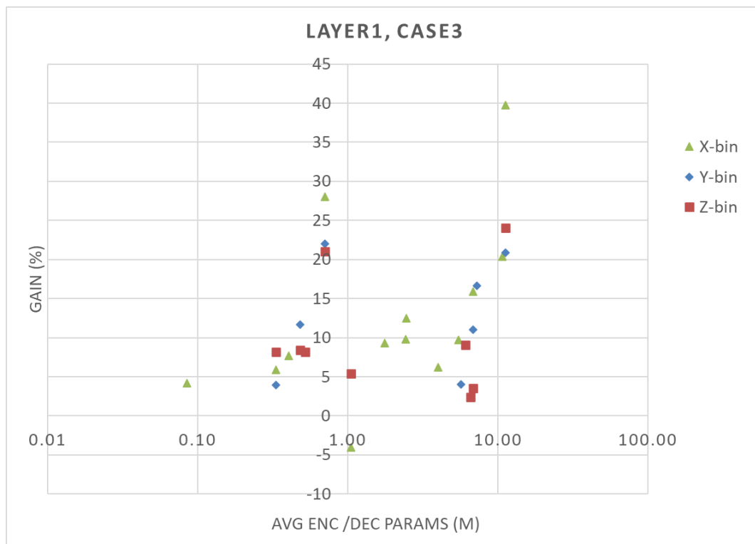
Figure 6.2.2.18-15: Case 3, model size (#parameters) vs. SGCS gain
