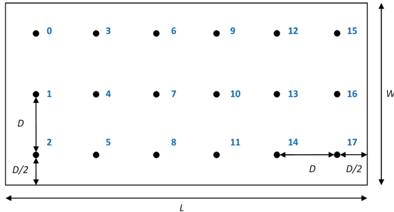
Figure 6.4.1-5: TRP layout and their indices for the evaluation of AI/ML based positioning.
