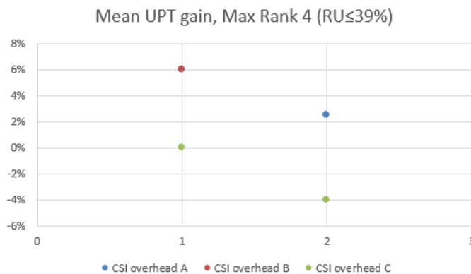
Figure 6.2.2.8-3: Mean UPT gain, Max Rank 4 (RU≤39%), x-axis means index of source
