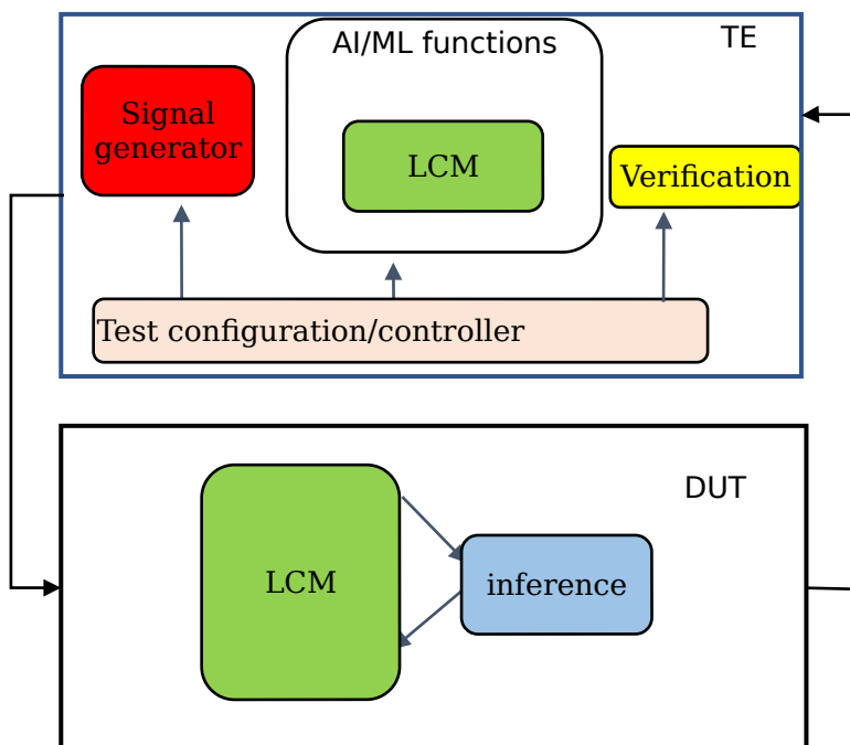
Figure 7.3.2.3-1: Reference block diagram for 1-sided model
