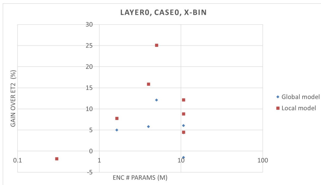
Figure 6.2.2.18-18: Case 0 model size (#paramters) vs. SGCS gain for global and local models
