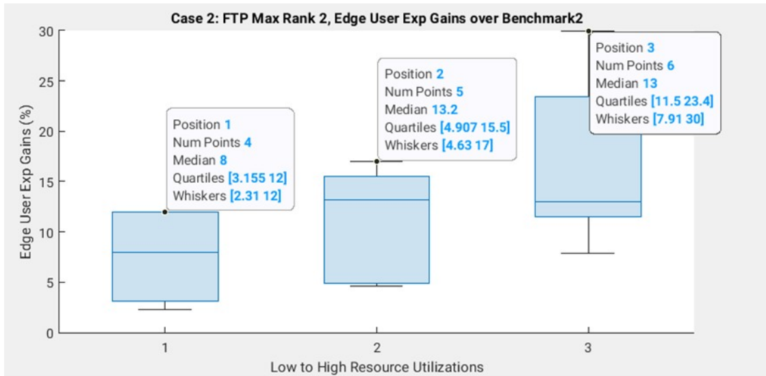
Figure 6.2.2.9-8: Median, 0.75 quantile, 0.25 quantile, outliers, and min/max values excluding outliers for “A” CSI payload bins for various resource utilizations
