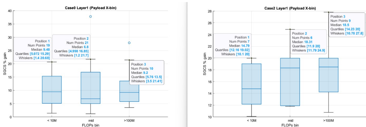
Figure 6.2.2.18-13: Alternative visualization of Case 0 and Case 2 comparison in terms of complexity vs. performance
