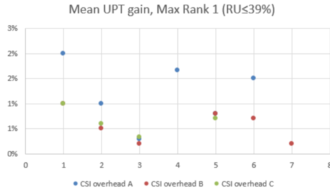
Figure 6.2.2.8-1: Mean UPT gain, Max Rank 1 (RU≤39%), x-axis means index of source
