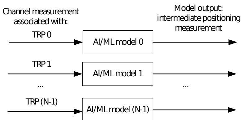
Figure 6.4.1-4: Assisted positioning with single-TRP construction, and N models for N TRPs.
