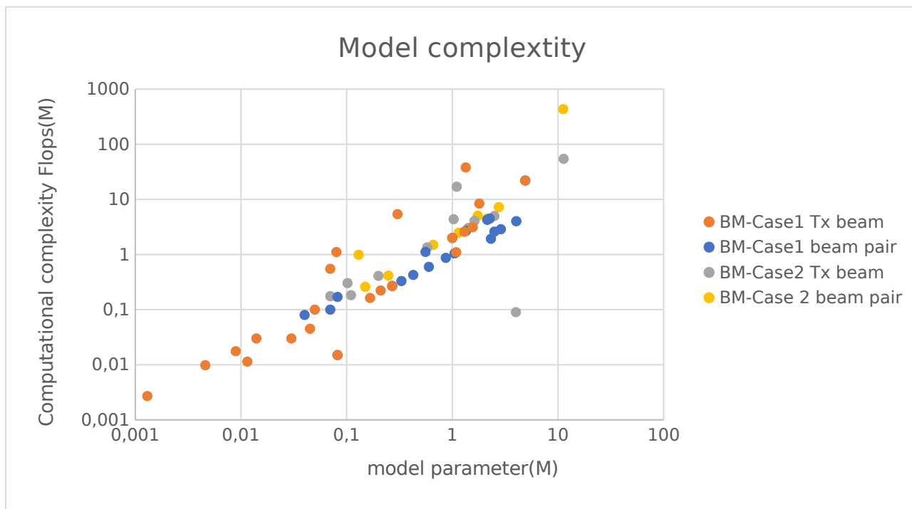
Figure 6.3.2-1: Complexity of AI/ML models from evaluation results in terms of FLOPs and number of parameters for BM cases
