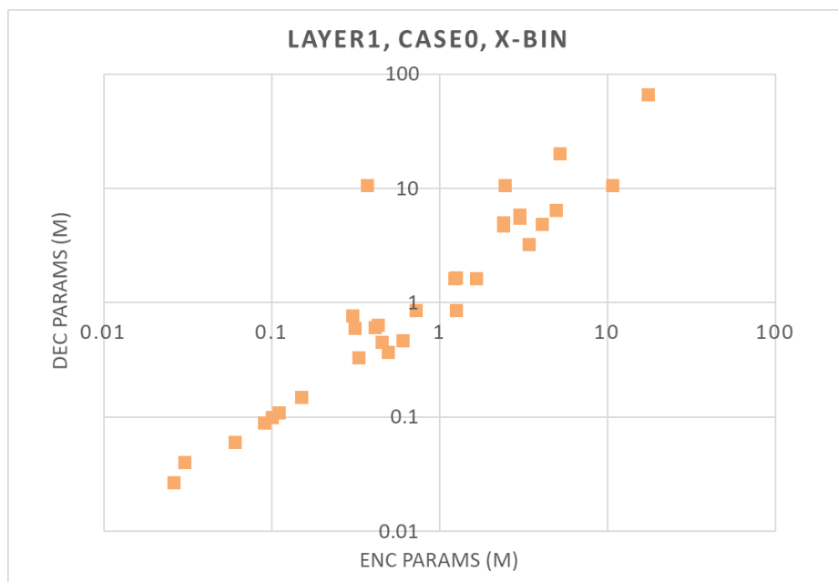
Figure 6.2.2.18-8: Decoder model size vs. Encoder model size (#parameters)
