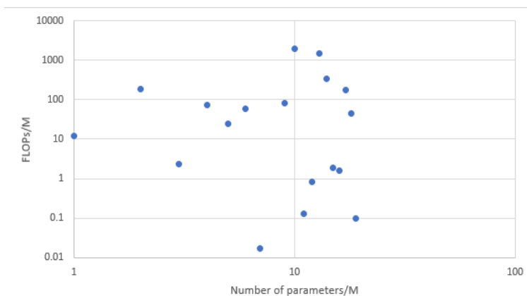
Figure 6.2.2.6-1: Complexity of AI/ML models from evaluation results in terms of FLOPs and number of parameters for CSI prediction.
