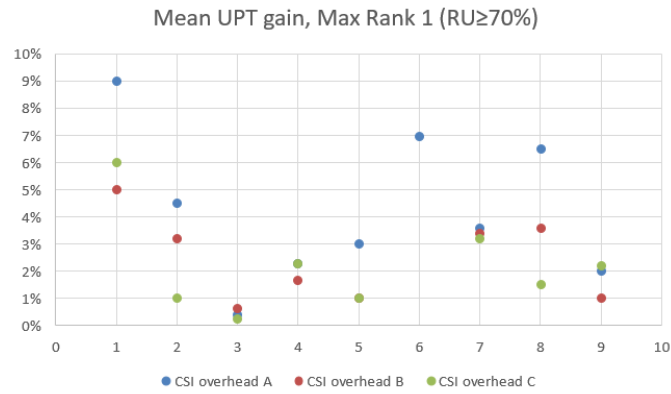
Figure 6.2.2.8-7: Mean UPT gain, Max Rank 1 ( RU \geq 70\% ), x-axis means index of source
