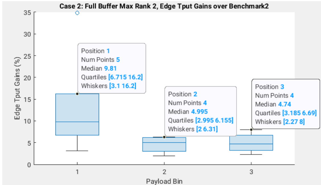
Figure 6.2.2.9-12: Edge Throughput gains over Benchmark 2, for Bins A, B and C, for Max Rank =2
