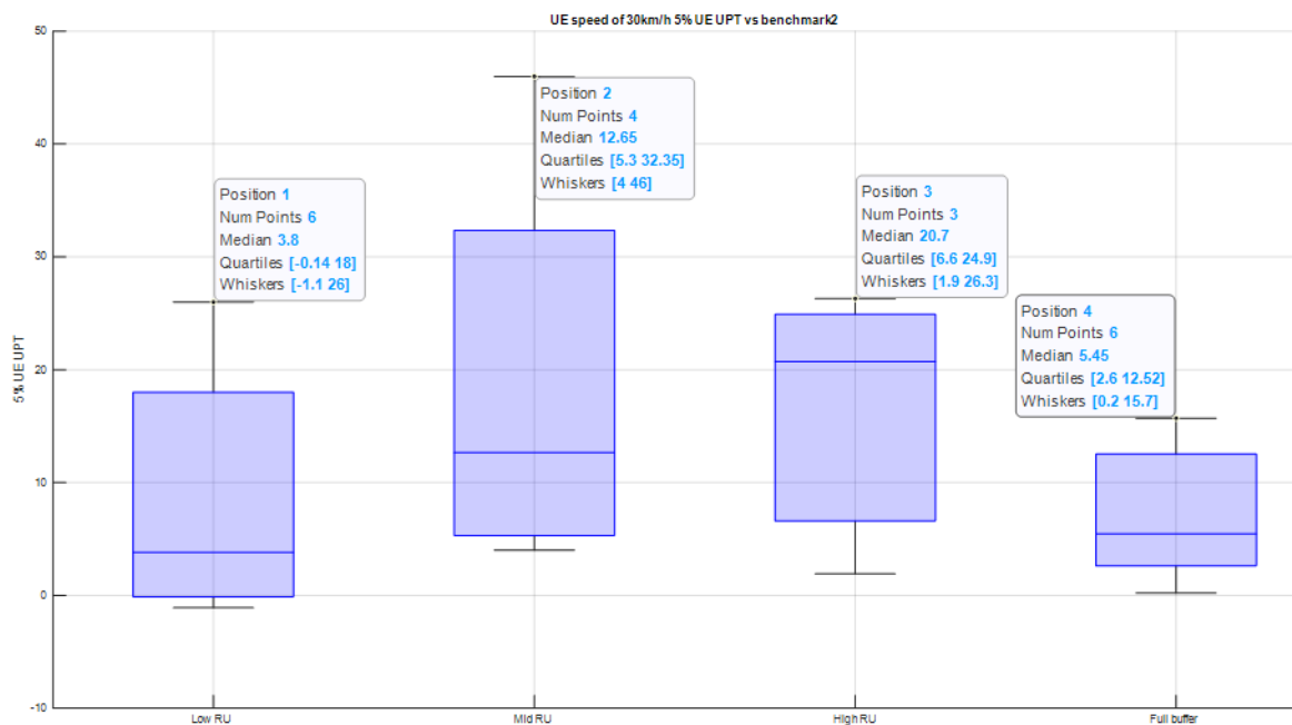
Figure 6.2.2.6A-4: 5% UPT distributions for full buffer with UE speed of 30km/h.
