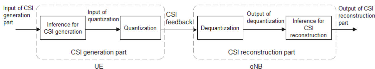
Figure 6.2.1-1: An example of the CSI compression inference procedure
