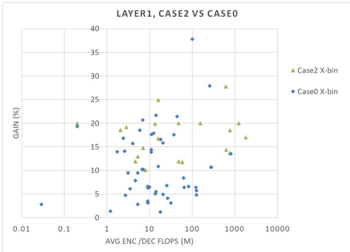
Figure 6.2.2.18-12: Case 0 compared to Case 2 in terms of complexity vs. performance
