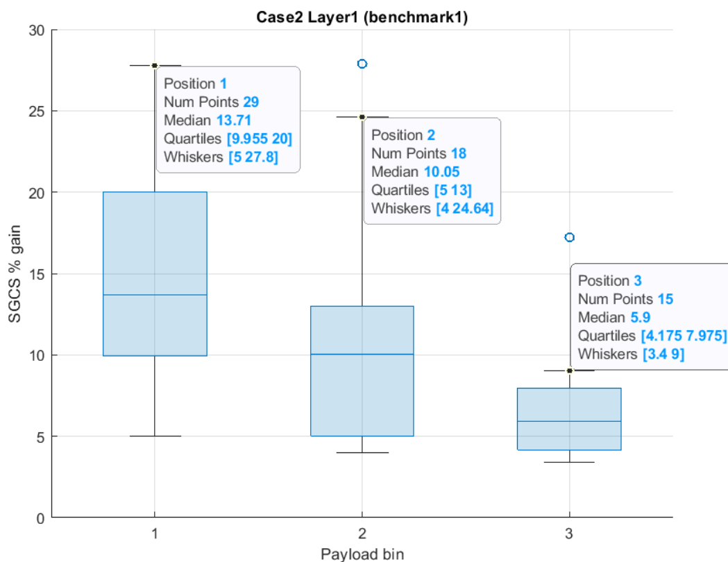
Figure 6.2.2.9-1: SGCS gain Case 2, Layer 1 for benchmark 1
