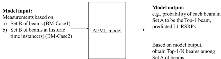
Figure 6.3.1-1: An example of the inference procedure for beam management.
