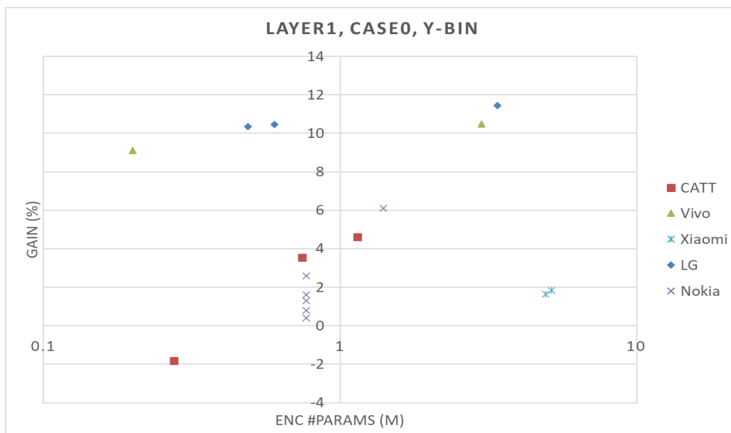
Figure 6.2.2.18-5: Case 0, encoder model size (#paramters) vs. SGCS gain (Y-bin)
