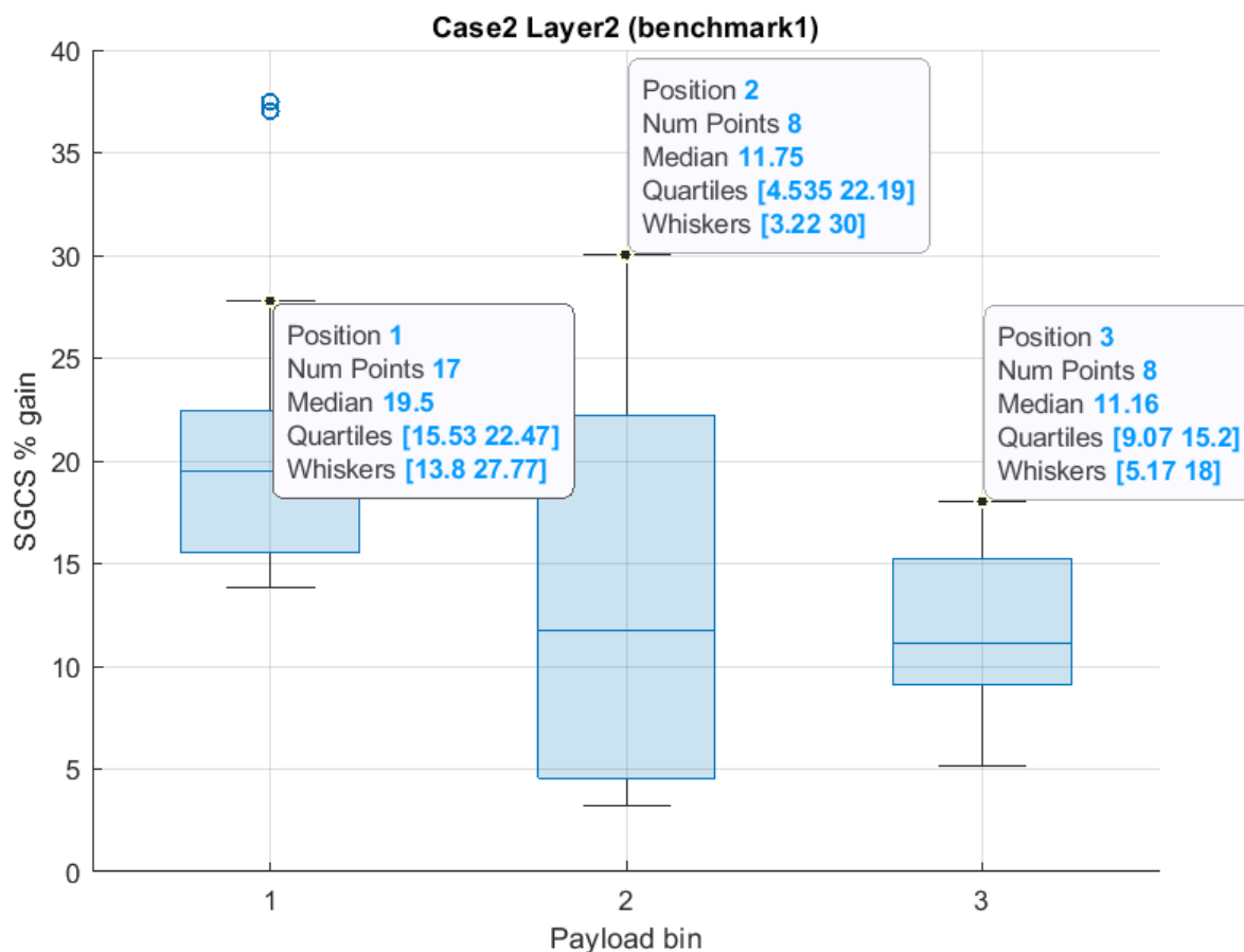
Figure 6.2.2.9-2: SGCS gain Case 2, Layer 2 for benchmark 1
