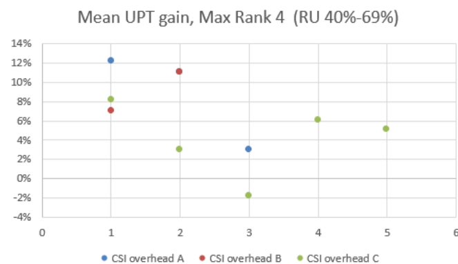
Figure 6.2.2.8-6: Mean UPT gain, Max Rank 4 (RU40%-69%), x-axis means index of source
