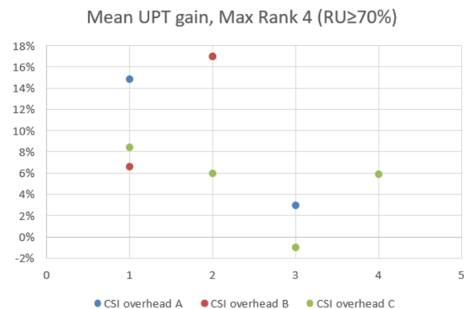
Figure 6.2.2.8-9: Mean UPT gain, Max Rank 4 ( RU \geq 70\% ), x-axis means index of source
