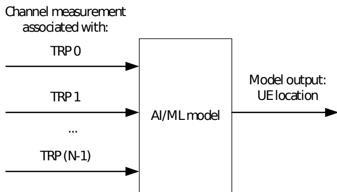
Figure 6.4.1-1: Direct AI/ML positioning
