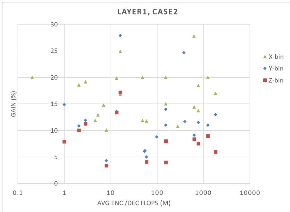
Figure 6.2.2.18-10: Case 2, model complexity (FLOPs) vs. SGCS gain
