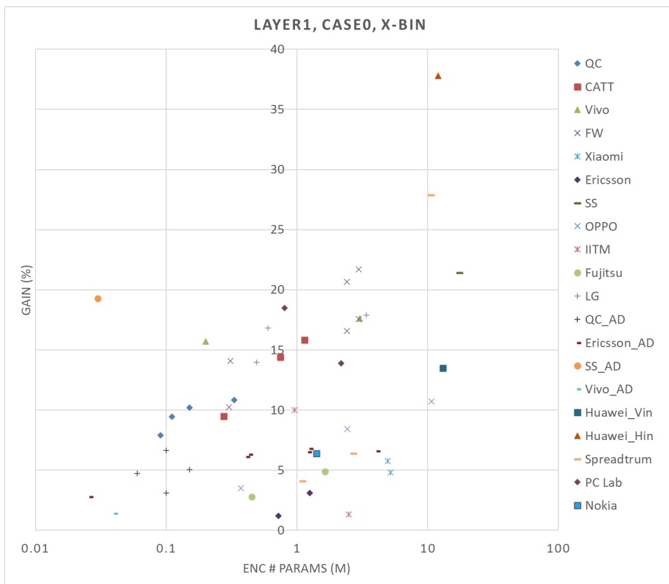
Figure 6.2.2.18-4: Case 0, encoder model size (#paramters) vs. SGCS gain (X-bin)
