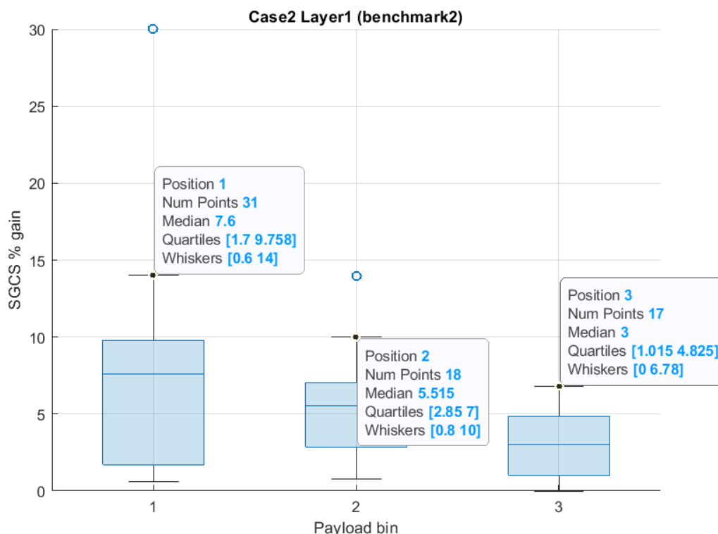
Figure 6.2.2.9-3: SGCS gain Case 2, Layer 1 for benchmark 2
