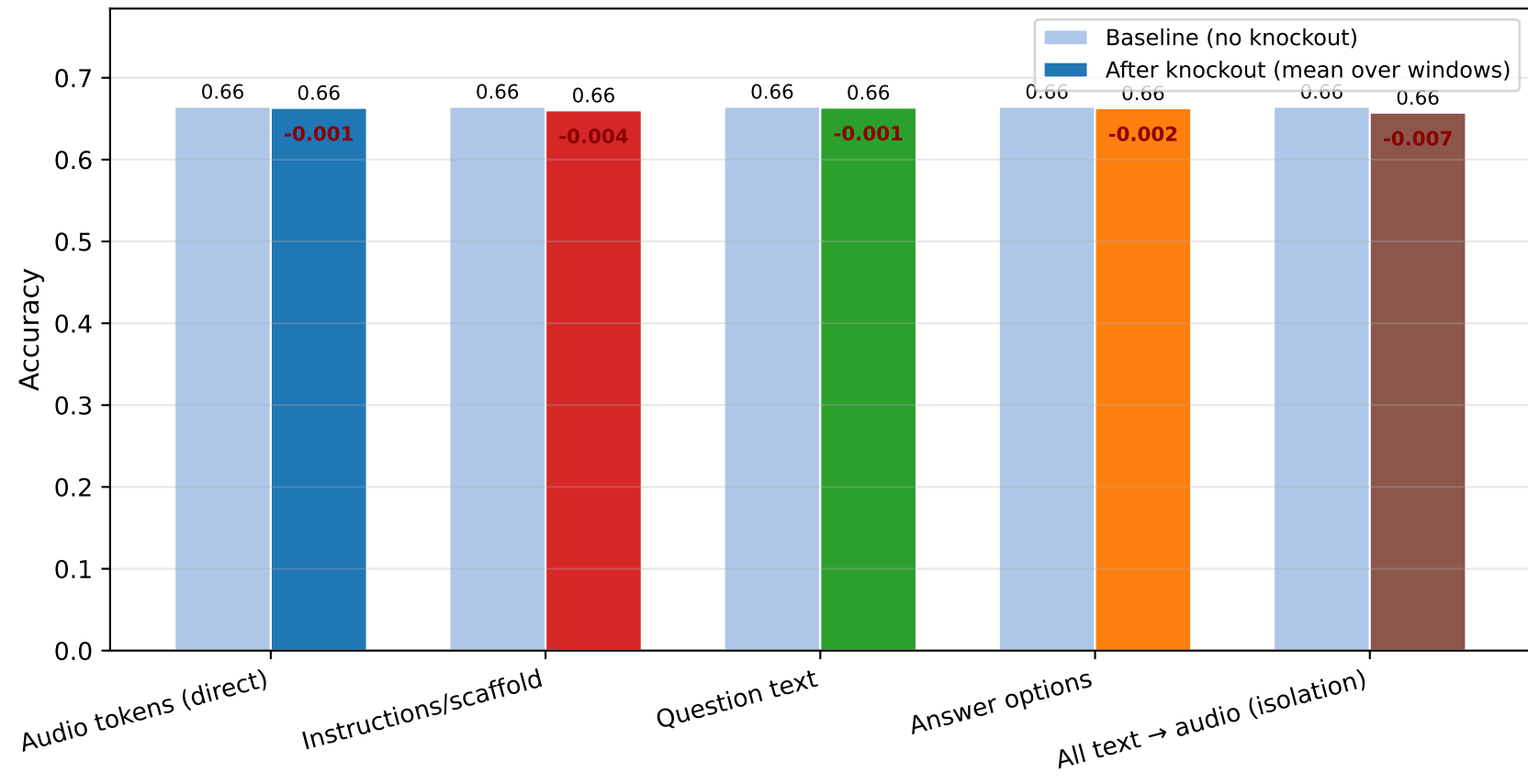
Experiment 2 — Accuracy Before and After Attention Knockout (knockout: source → component; averaged over all layer windows)
