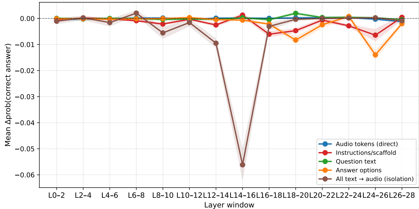
Experiment 2 — Knockout Effect per Layer Window (decision → component; lower = component more important in that window (shaded band = \pm SEM))
