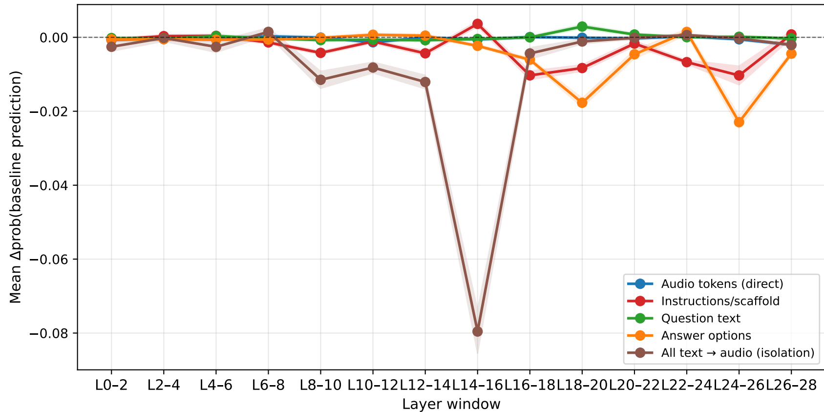
Experiment 2 — Knockout Effect per Layer Window — position-bias-immune (decision → component; lower = component more important in that window (shaded band = \pm SEM))
