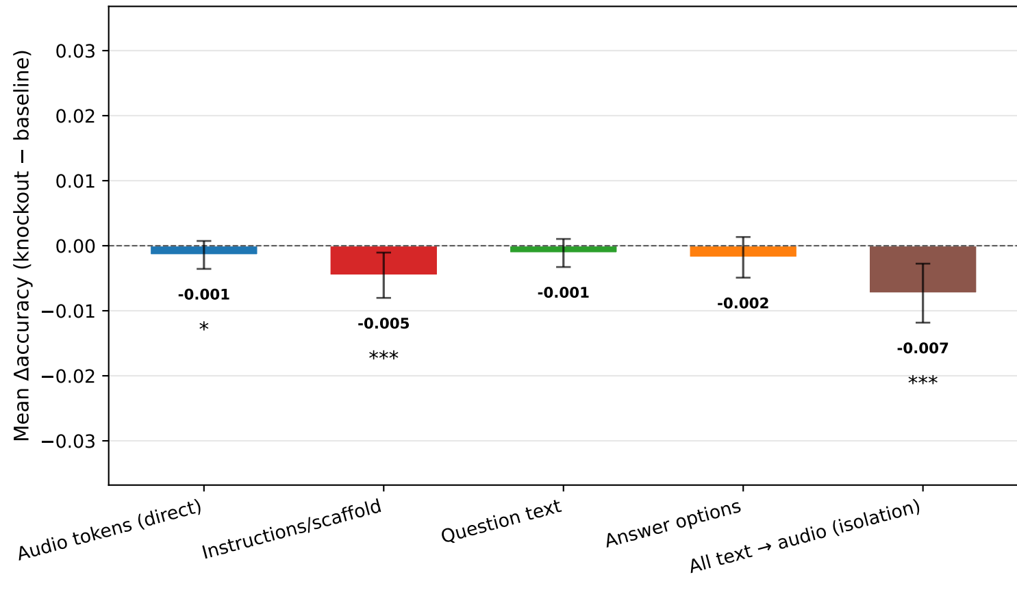
Experiment 2 — Attention Knockout: Effect on Answer (n=960 evals, averaged over all layer windows; error bars=SEM; * p<.05 ** p<.01 *** p<.001)
