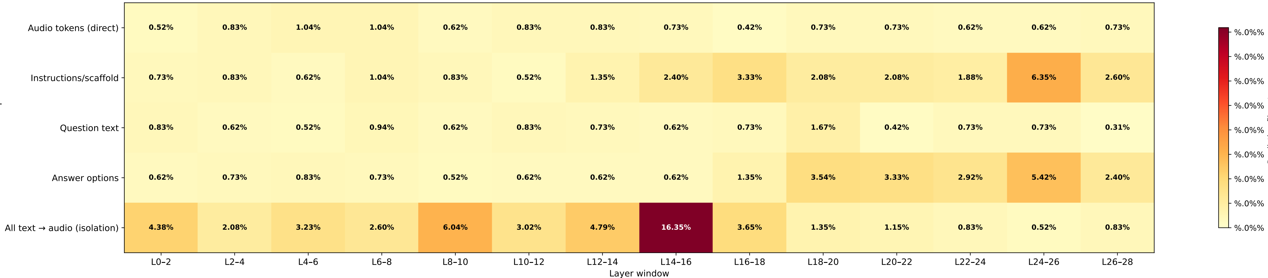
Experiment 2 — Prediction Flip Rate by Component × Layer Window (fraction of eval items where knockout changed the predicted answer)
