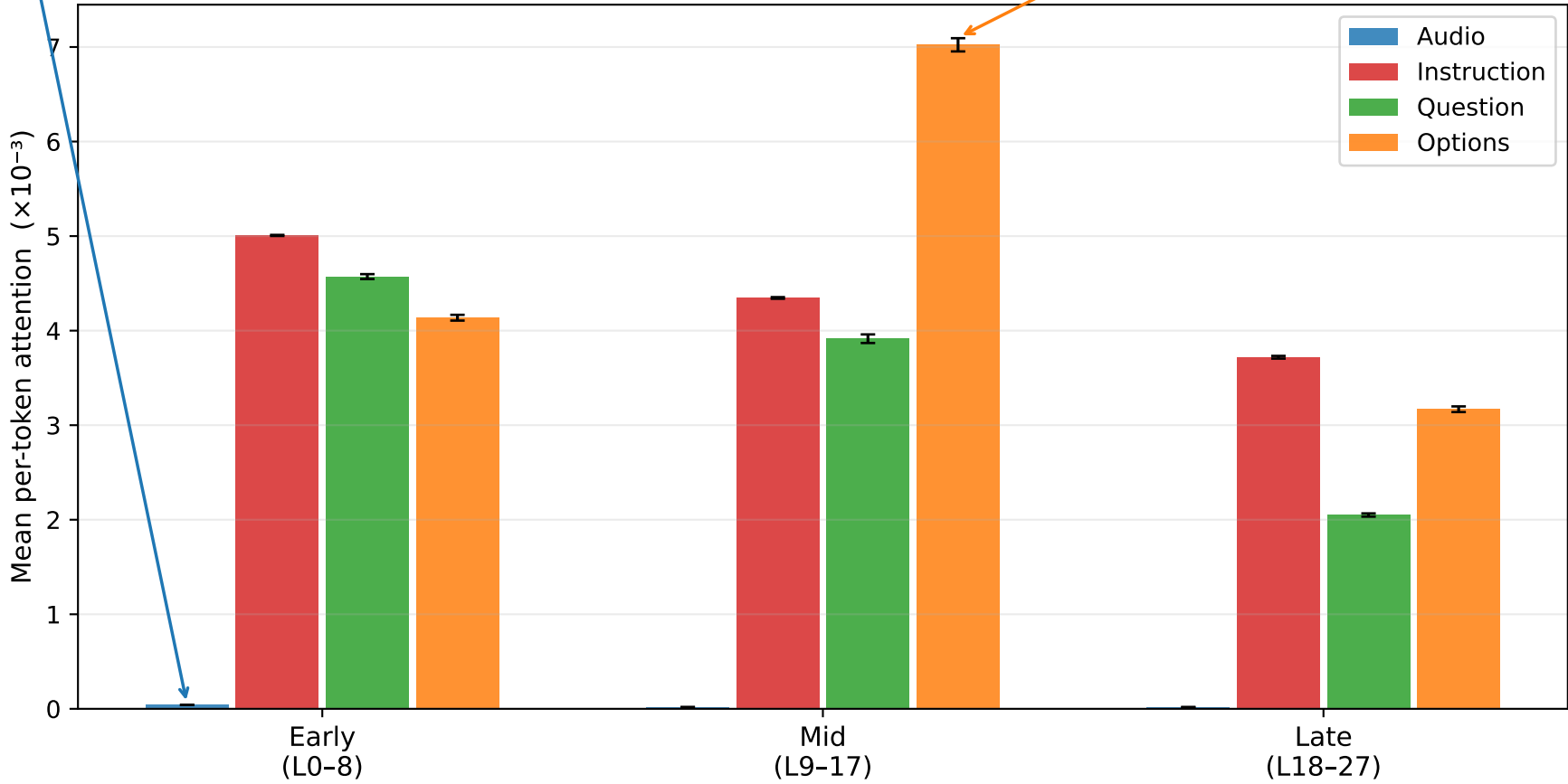
Experiment 1 — Per-token attention by processing phase (excl. other_text; Qwen2.5-Omni-7B, HumMusQA)
