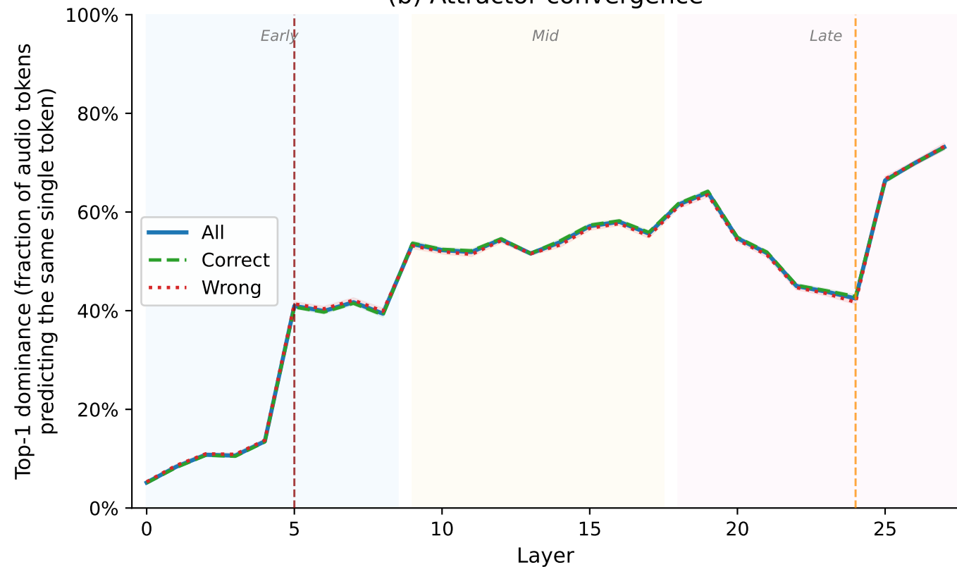
(b) Attractor convergence
