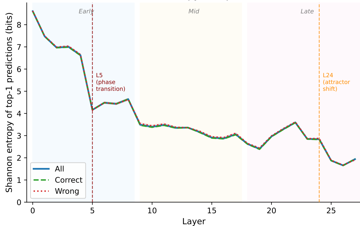
(a) Entropy collapse
