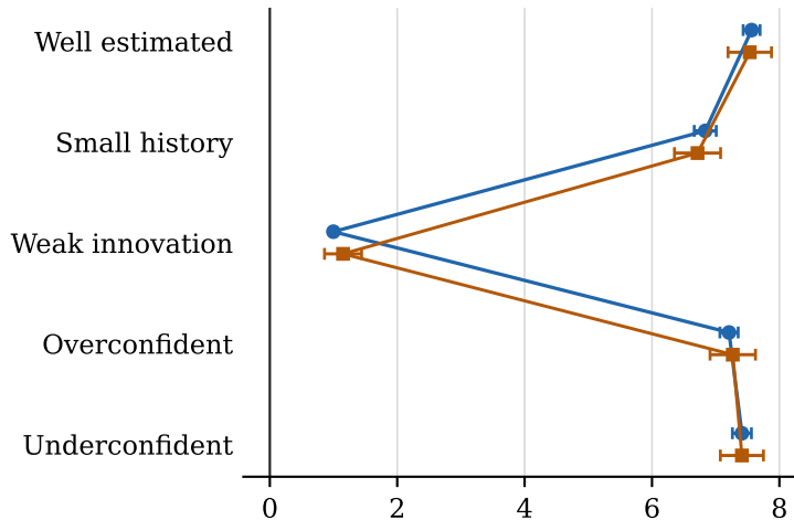
NFR interpolation weight \alpha = 0.0
