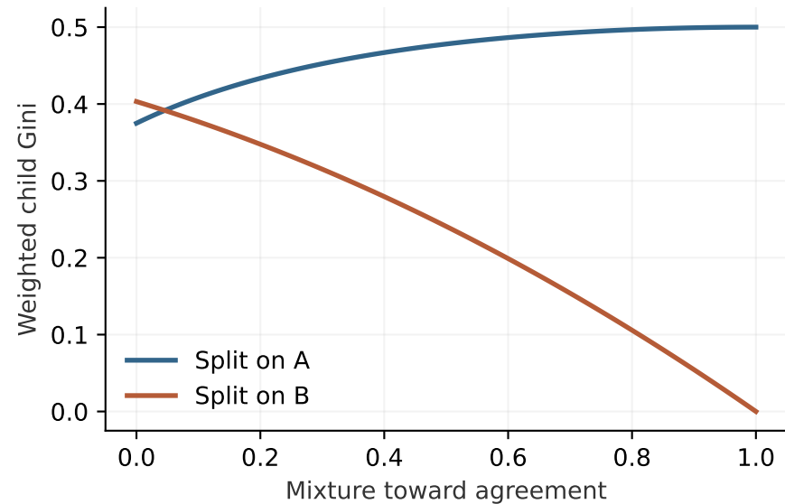
Gini and classification error can favor different splits
