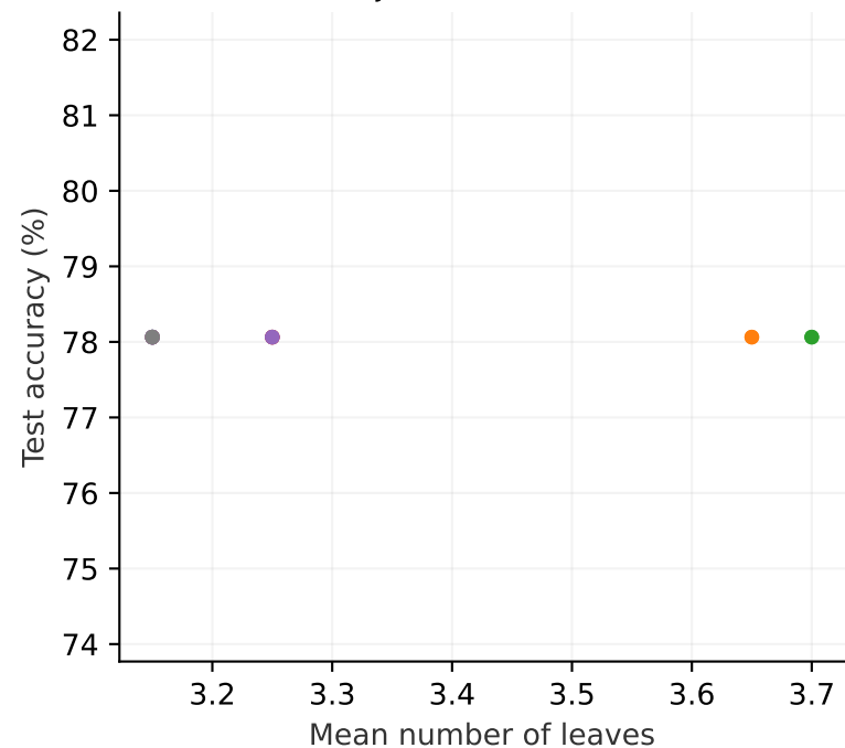
Objective, n = 800
