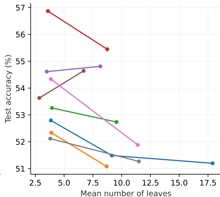
Noise, n = 200
