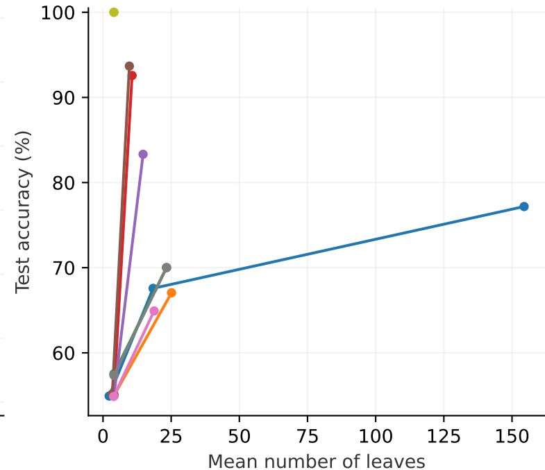
Interaction, n = 800
