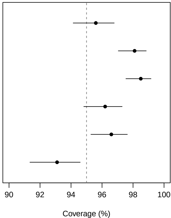
Normal interval coverage
