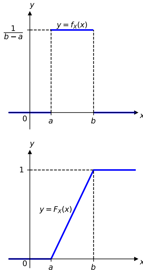
Figure 2: Graphs of PDF and CDF of X \sim U(a, b) .
