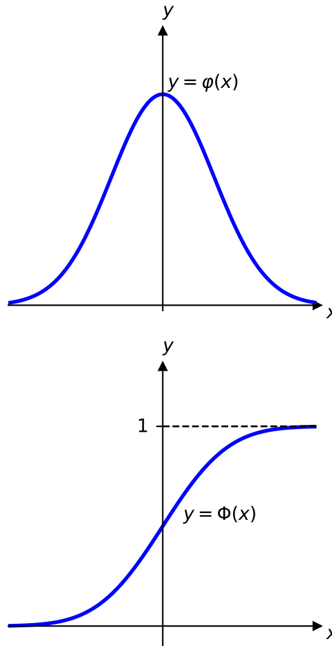
Figure 5: Functions \varphi(x) and \Phi(x)
