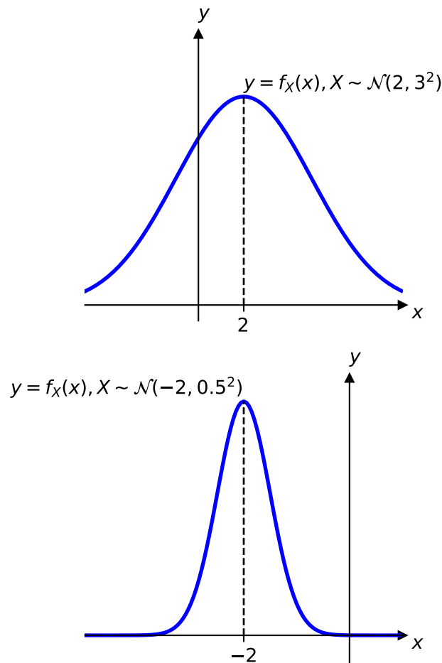
Figure 4: Graphs of PDF of X \sim \mathcal{N}(2, 3^2) and X \sim \mathcal{N}(-2, 0.5^2) .
