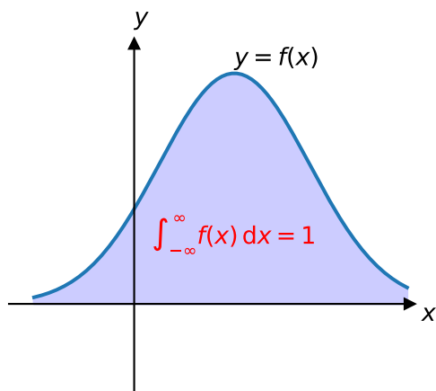
Figure 1: Visual representation of probabilities for a continuous random variable
