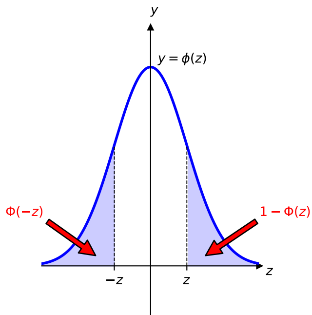
Figure 6: Illustration that \Phi(-z) = 1 - \Phi(z)
