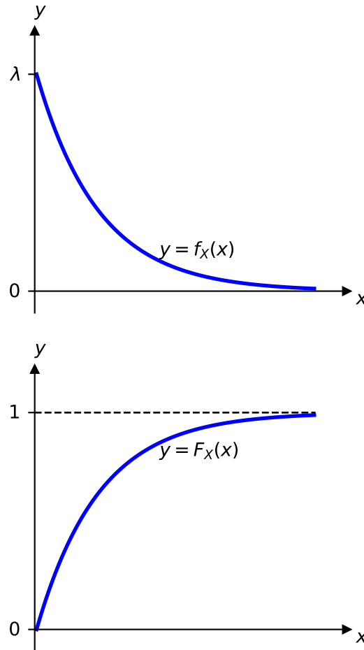
Figure 3: Graphs of PDF and CDF of X \sim \text{Exp}(\lambda) . Graphs are shown for x \geq 0 only. Both functions equal 0 for x < 0 .
