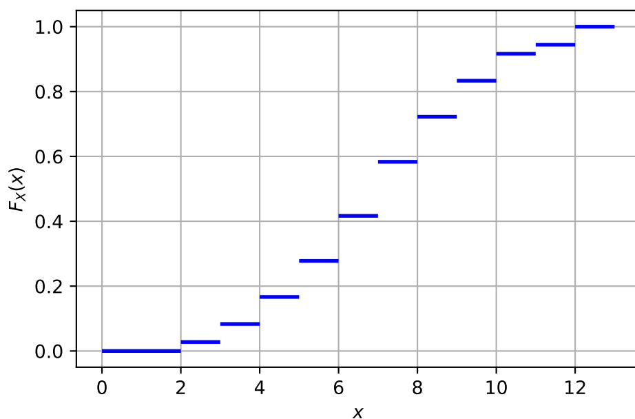
Figure 2: Cumulative distribution function of the sum of two fair dice
