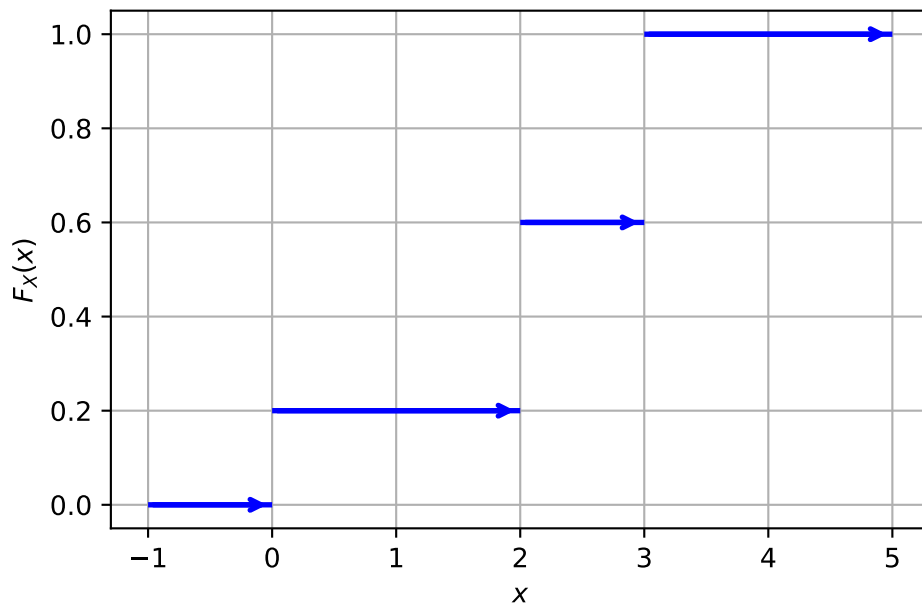
Figure 1: Cumulative function of the random variable X : \Omega \rightarrow \{0, 2, 3\} with \mathbb{P}(X = 0) = 0.2 , \mathbb{P}(X = 2) = \mathbb{P}(X = 3) = 0.4
